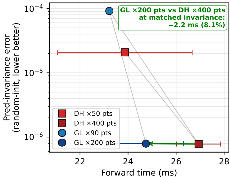
QM9-small (4L / 64ch / lmax=4 / mmax=2)
