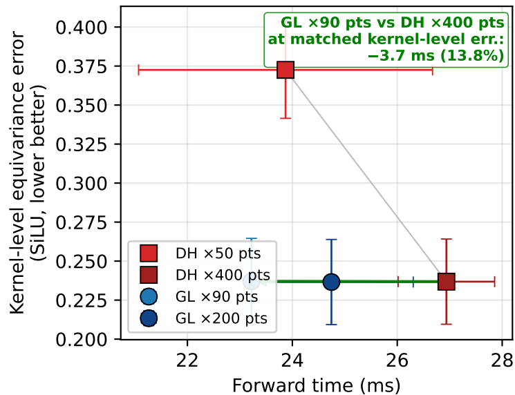
QM9-small (4L / 64ch / lmax=4 / mmax=2)
