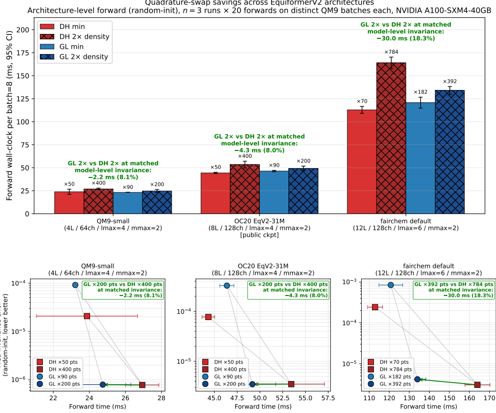
Figure 3: (top) Forward wall-clock per QM9 batch 8 across three EquiformerV2 architectures, for four grid configurations. n = 3 runs \times 20 measured forwards on distinct batches per run, error bars 95% CI on run means. Architecture-level (random-init) timing. (bottom) Model-level prediction-invariance error vs. forward time for the same configurations. Pred-invariance is \mathbb{E}_{R,x} |f(x) - f(Rx)|/|f(x)| at random-init weights, 10 SO(3) rotations \times 20 distinct QM9 batches per cell. Both 2 \times grids reach \sim 10^{-6} pred-invariance; GL match-DH (the matched-equivariance config in fig:pareto) tracks near DH default rather than near DH 2 \times , because at m_{\max} < \ell_{\max} the model-level error compounds the per-layer aliasing that the kernel-level metric does not see. Green arrows mark the wall-clock saved going DH 2 \times \rightarrow GL match-DH.
