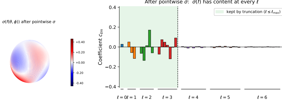
Figure 1: The S^2 -activation pipeline and the source of its equivariance error. (a) The four-stage operator \mathcal{A}_\sigma implemented in EquiformerV2’s S2Activation.forward : SH coefficients c are projected to grid values f(\theta_i, \phi_i) ( to-grid ), \sigma is applied pointwise on S^2 , and the result is integrated against w_i Y_{\ell m} to produce new SH coefficients c' ( from-grid ). Stages 1–3 are exact and equivariant; only the final integration is approximated, and the gap between the exact integral \int_{S^2} \sigma(f) Y_{\ell m} d\Omega and the finite-quadrature sum \sum_i w_i \sigma(f(\theta_i, \phi_i)) Y_{\ell m}(\theta_i, \phi_i) is the sole source of S^2 -activation equivariance error (Appendix A); three node families are illustrated in Figure 2. (b, d) The function on the sphere before and after the pointwise nonlinearity, on a shared diverging colour scale: f and \sigma(f) look qualitatively similar in the spatial domain ( \sigma slightly attenuates the negative regions but otherwise preserves the geometry). (c, e) The same two functions in the spectral domain. Signed SH coefficients c_{\ell m} are drawn one bar per (\ell, m) pair, grouped by \ell with within-group ordering m = -\ell, \dots, +\ell (groups coloured by \ell ); the green band marks the \ell \leq \ell_{\max} region kept by the network’s truncation. (c) f has c_{\ell m} = 0 for \ell > \ell_{\max} . (e) \sigma(f) has nonzero c_{\ell m} at every \ell , with a tail that decays toward \ell \rightarrow \infty but never reaches zero. A finite grid cannot resolve that high- \ell tail, and the unresolved content aliases back into the kept coefficients in a rotation-dependent way – breaking equivariance.
