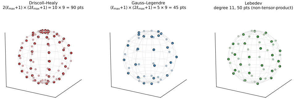
(b) Three quadrature node layouts on S^2 for \ell_{\max} = 4 . Driscoll-Healy uses an equiangular tensor-product grid with 2(\ell_{\max} + 1) latitude rings, twice what Gauss-Legendre needs for the same exactness. Lebedev avoids the tensor-product structure entirely, distributing roughly the same number of points more uniformly. All three are exact for spherical polynomials of degree \leq 2\ell_{\max} .
