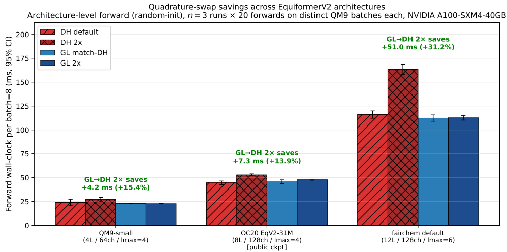
Figure 3: Forward wall-clock per QM9 batch 8 across three published EquiformerV2 architectures, for four grid configurations. n = 3 runs \times 20 measured forwards on distinct batches per run, error bars 95% CI on run means. Architecture-level (random-init) timing.
