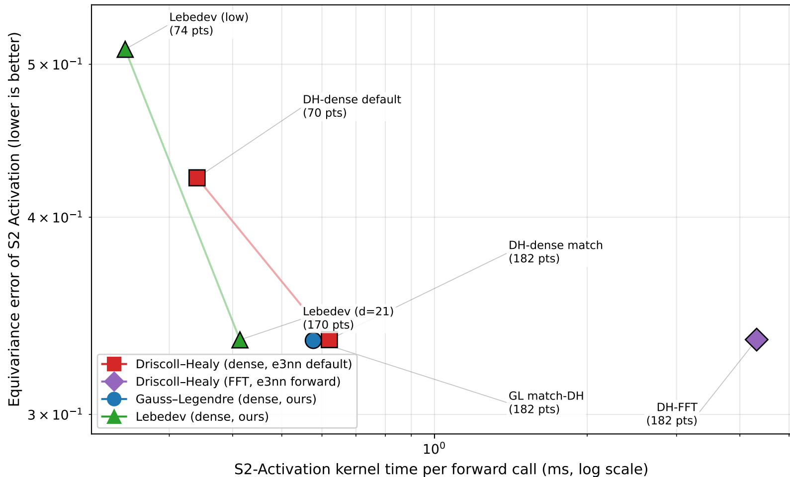
Kernel-level Pareto: 4 quadrature methods at \ell_{\max} = 6 , m_{\max} = 2 (S2-Activation alone, SiLU, batch=1024, 128 ch, A
