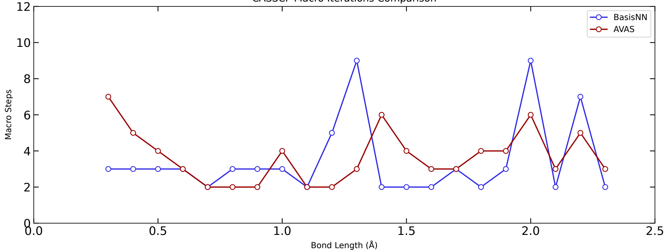
CASSCF Macro Iterations Comparison
