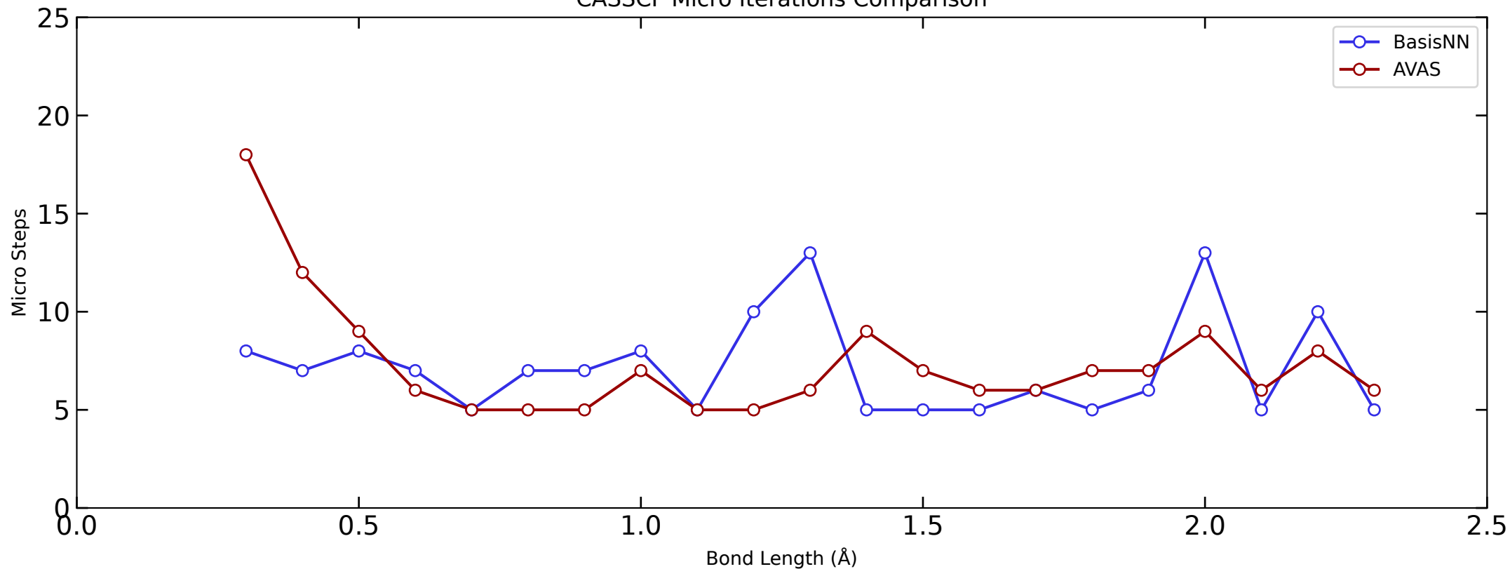
CASSCF Micro Iterations Comparison
