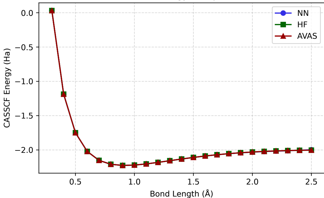
CASSCF Energy Comparison
