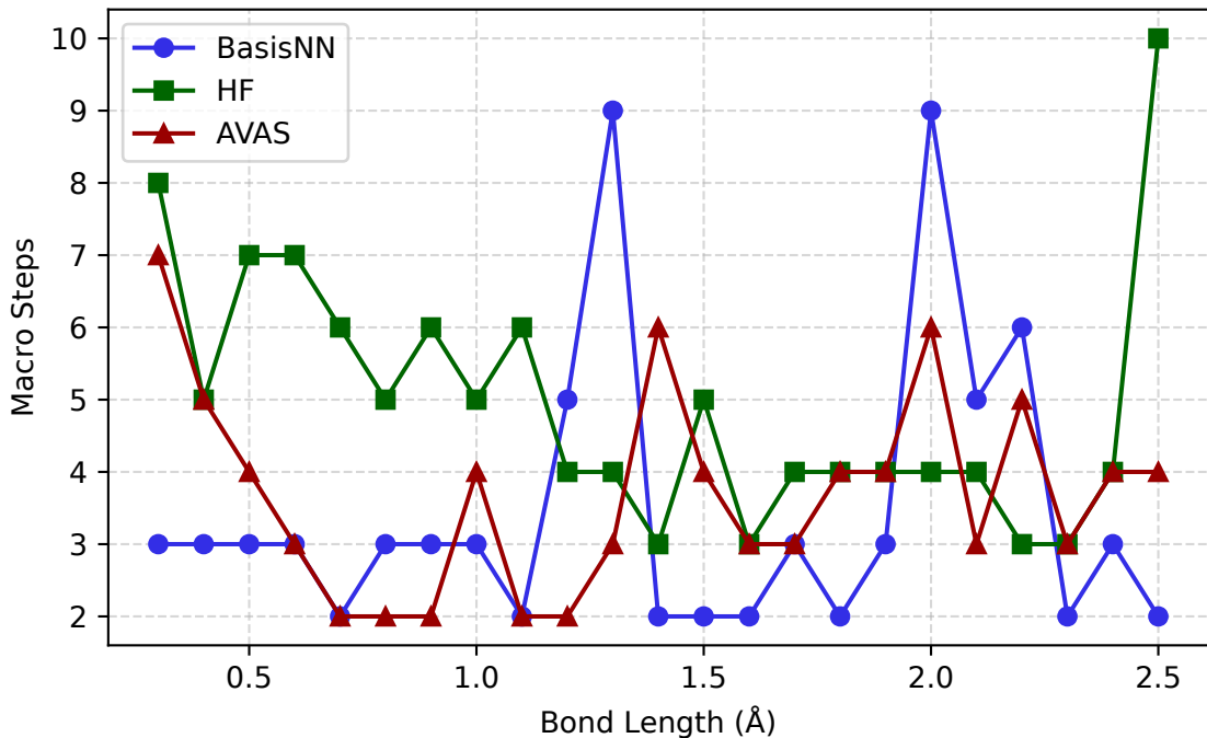
CASSCF Macro Iteration Comparison
