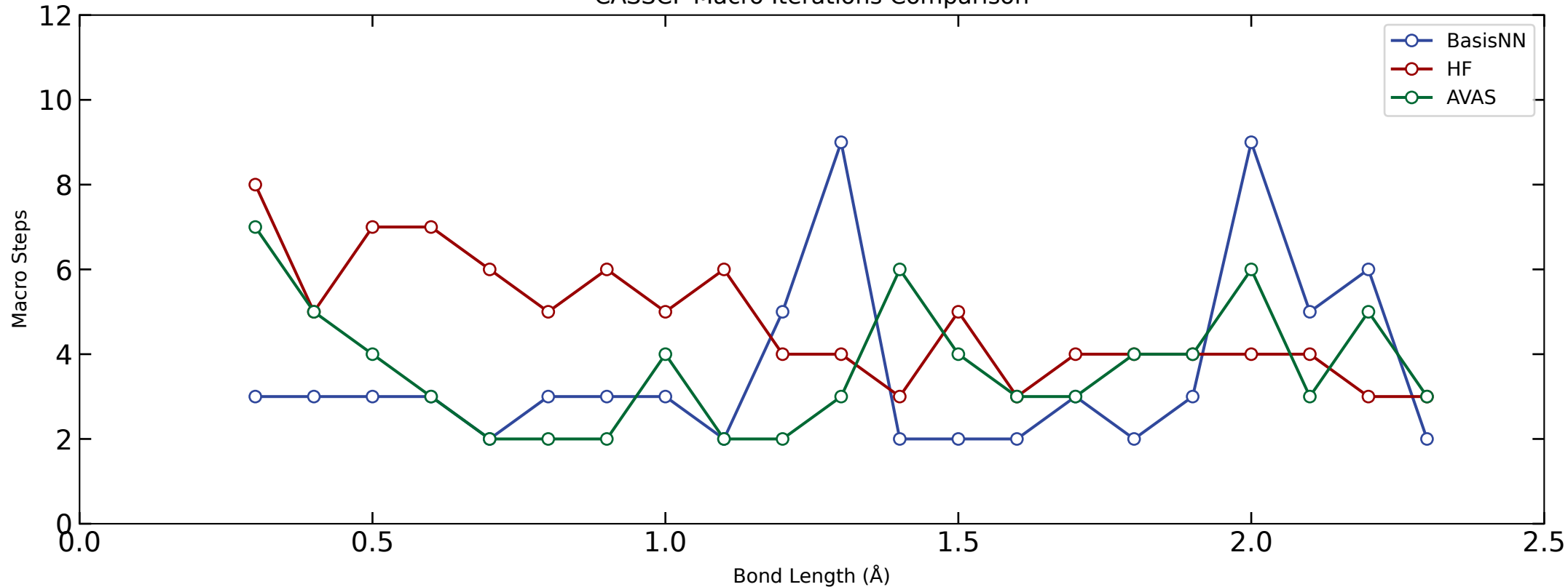
CASSCF Macro Iterations Comparison
