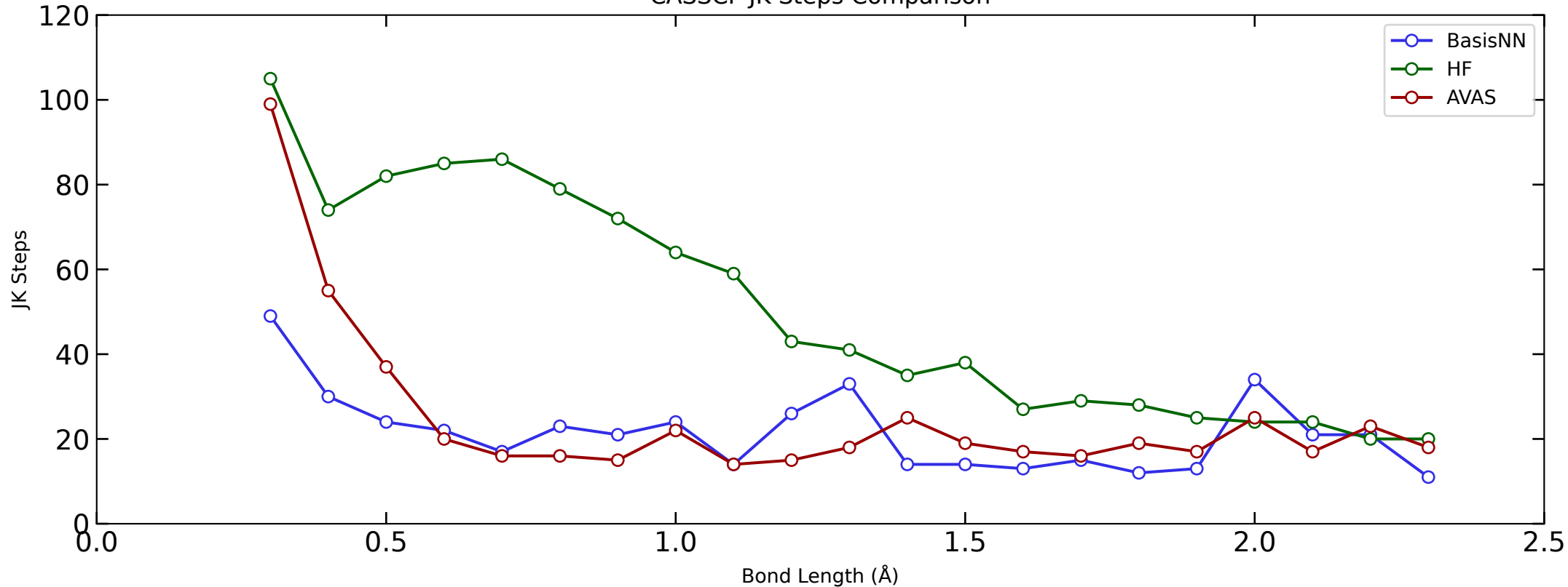
CASSCF JK Steps Comparison
