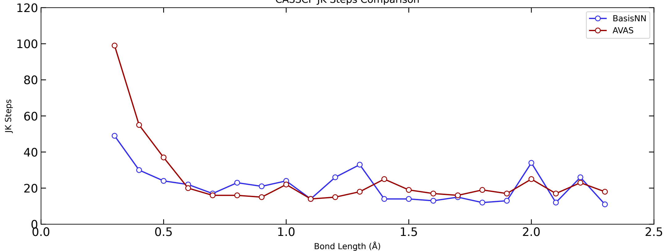
CASSCF JK Steps Comparison
