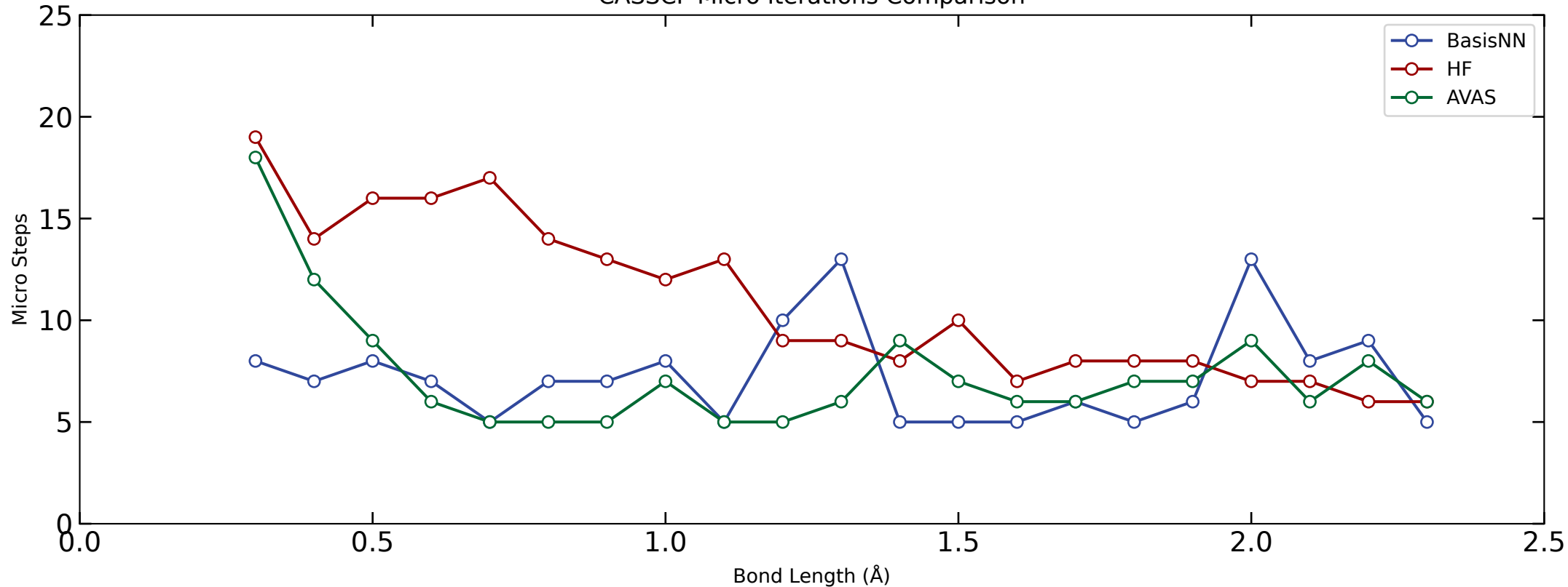
CASSCF Micro Iterations Comparison
