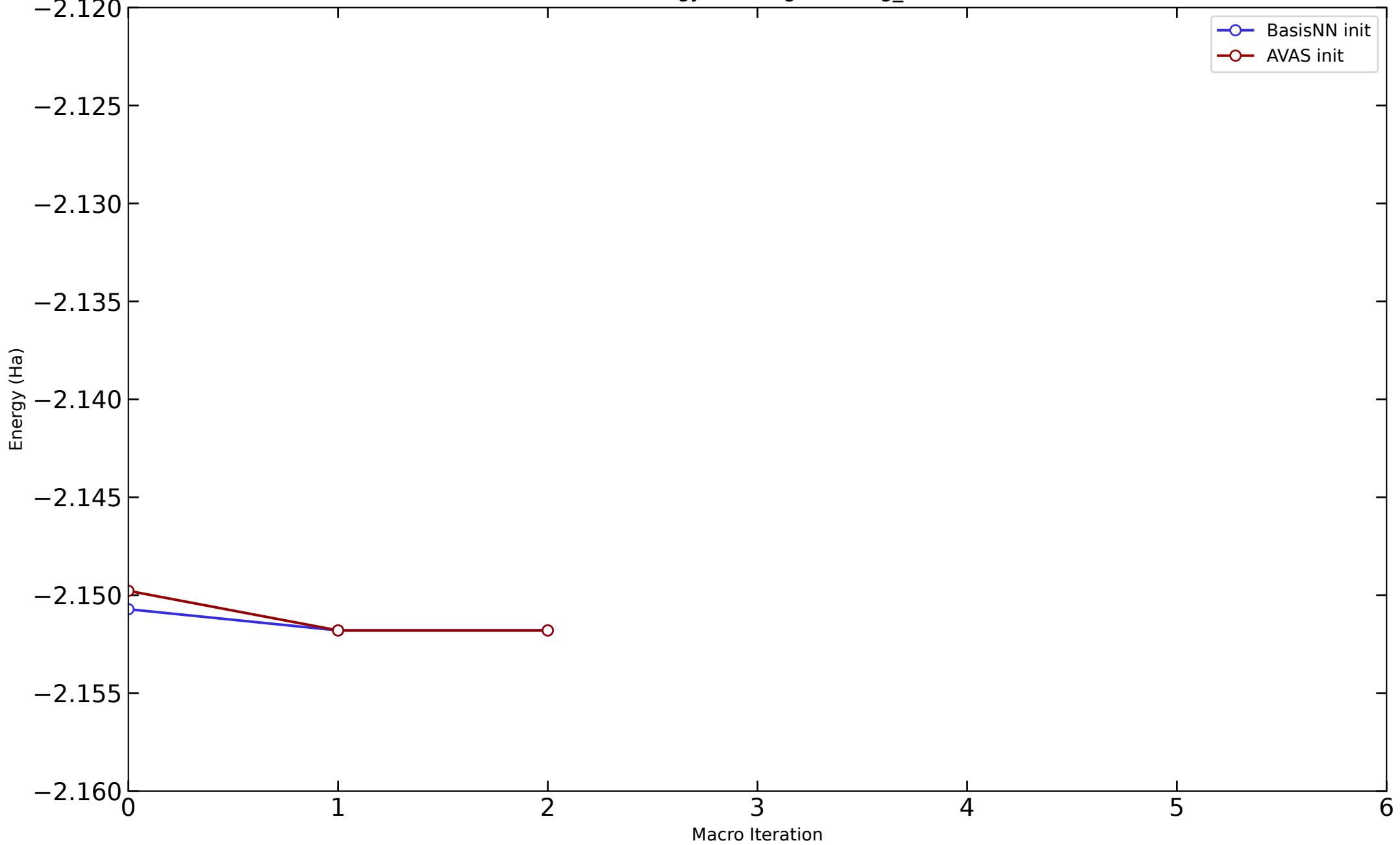
CASSCF Energy Convergence (log_22.txt)
