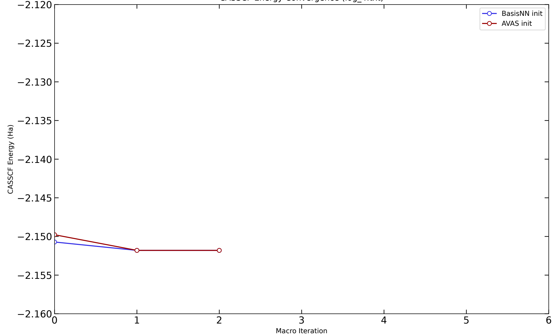
CASSCF Energy Convergence (log_4.txt)
