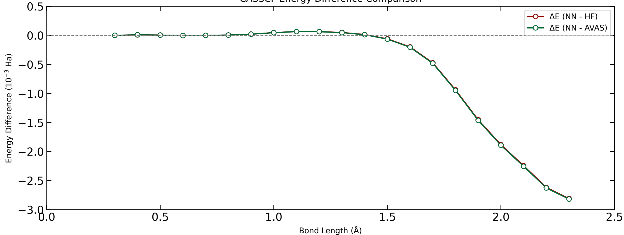
CASSCF Energy Difference Comparison
