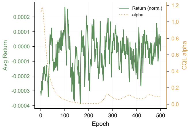
b Average Return & Lagrange alpha
