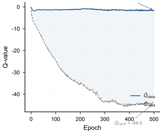
a Q-value Gap ( \Delta Q = 42 )
