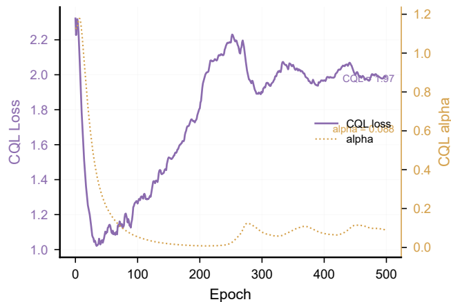
d CQL Penalty & Lagrange alpha
