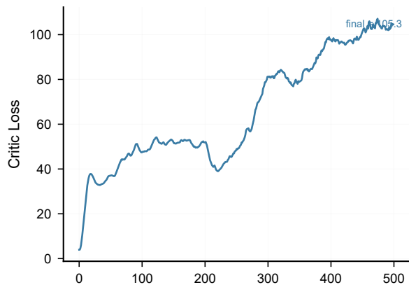
b Critic Total Loss
