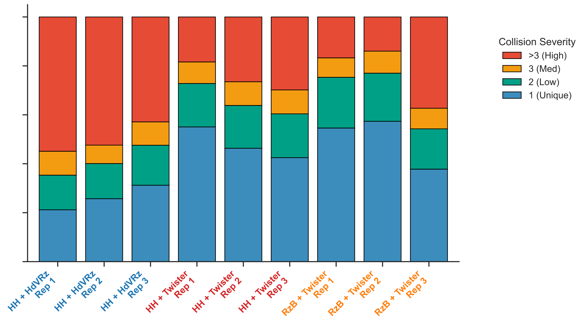
Brain Region: LGN
