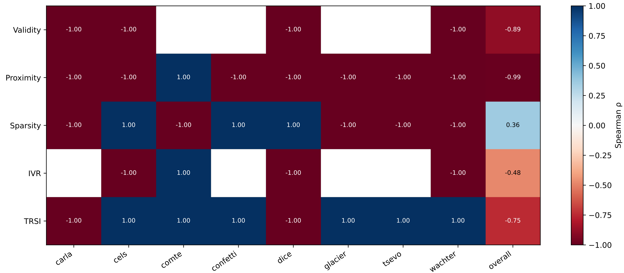
Fig 3: Spearman \rho — Traditional Metrics vs CF-faith
