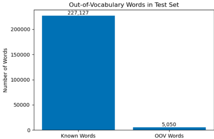
Figure 3: OOV word analysis on the test set.
