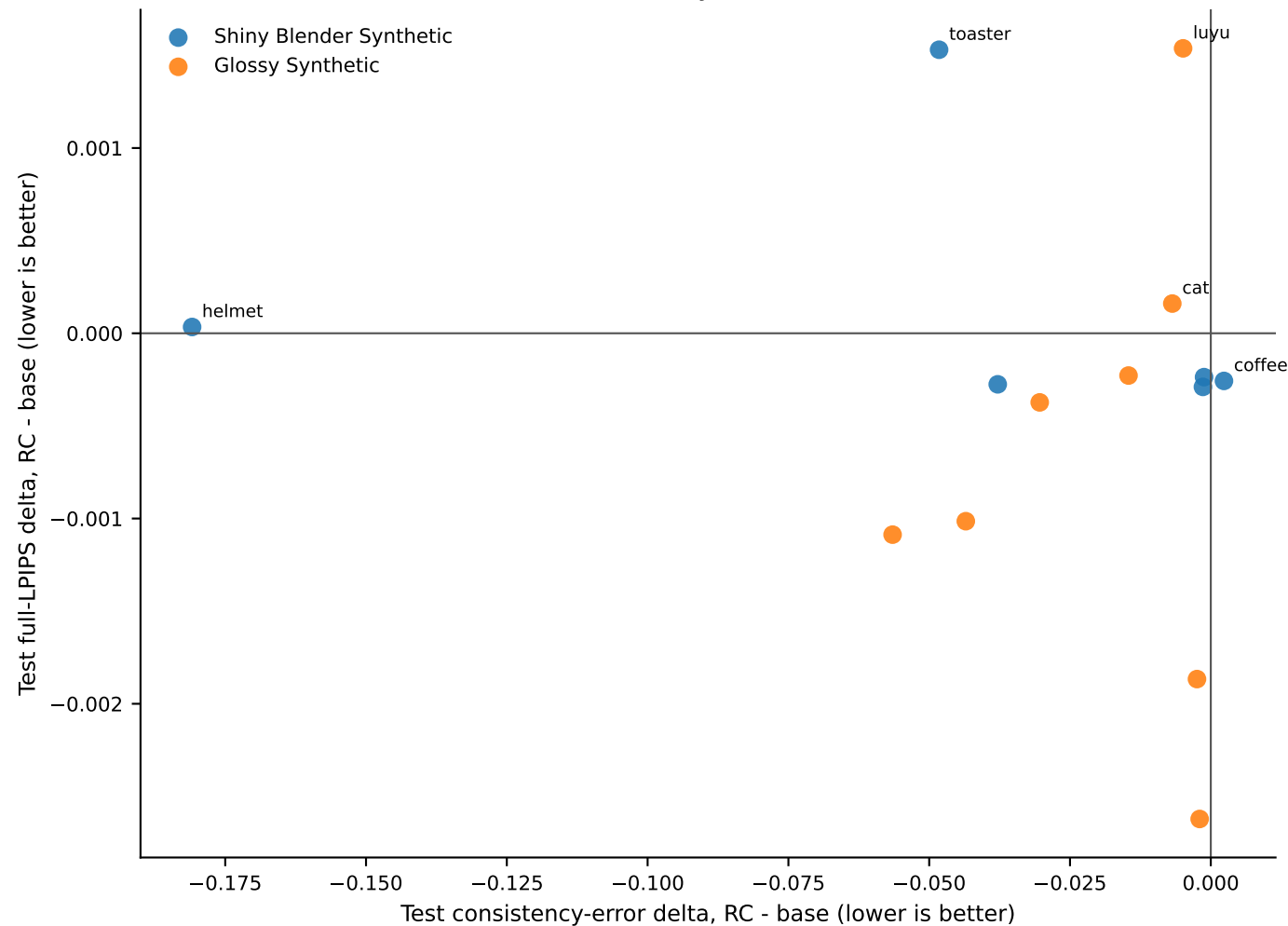
FD-P2-lite consistency vs full-LPIPS tradeoff
