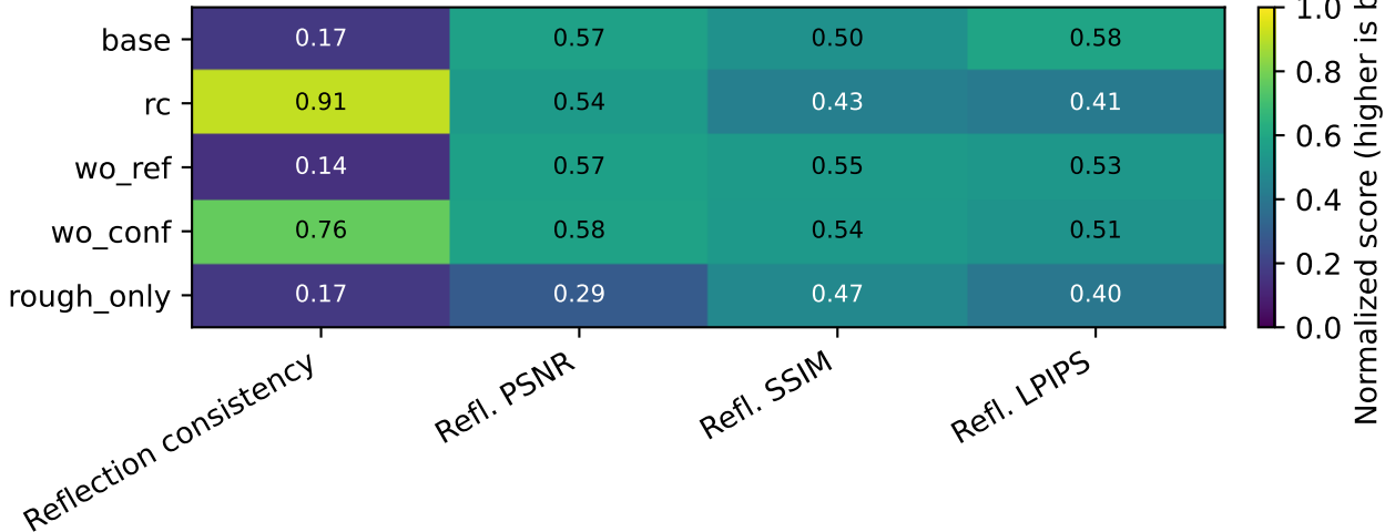
Ablation behavior on consistency and reflective metrics
