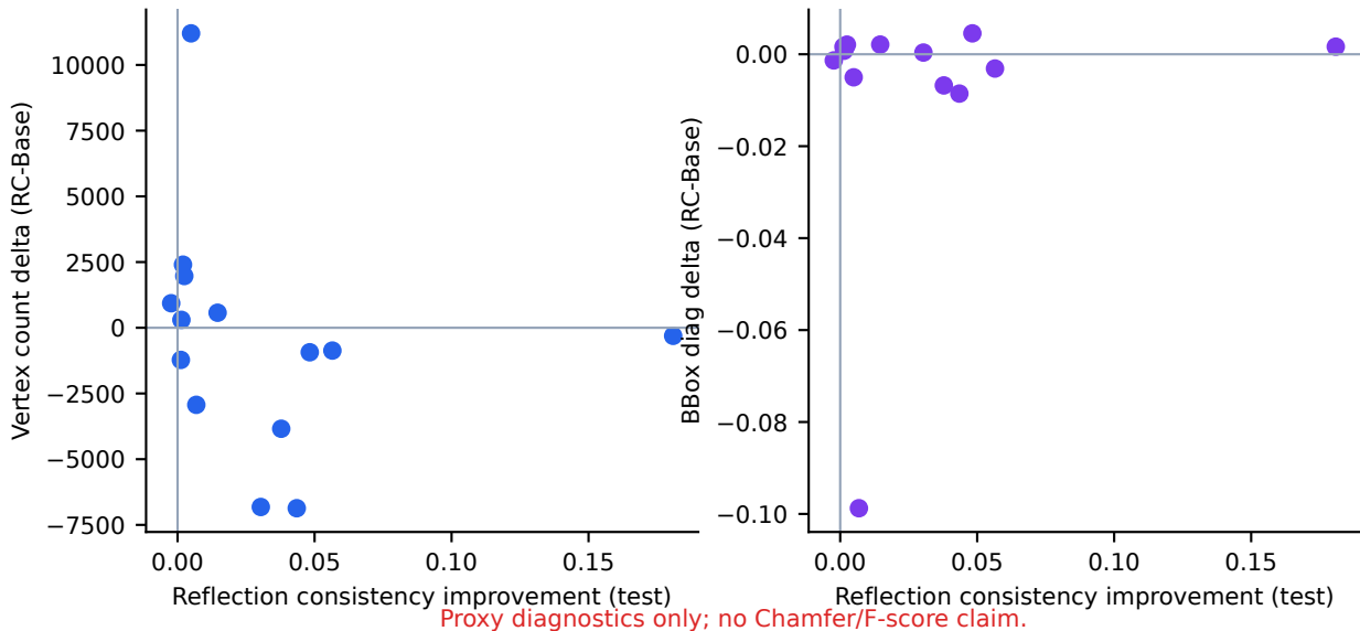
Fig. G2. Consistency vs geometry proxy trade-off
