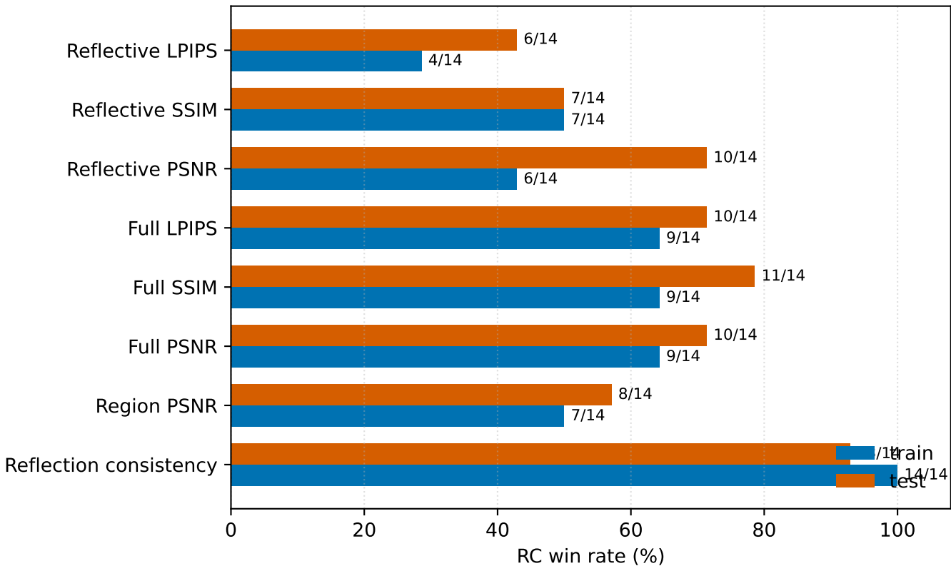
RC wins by metric and split
