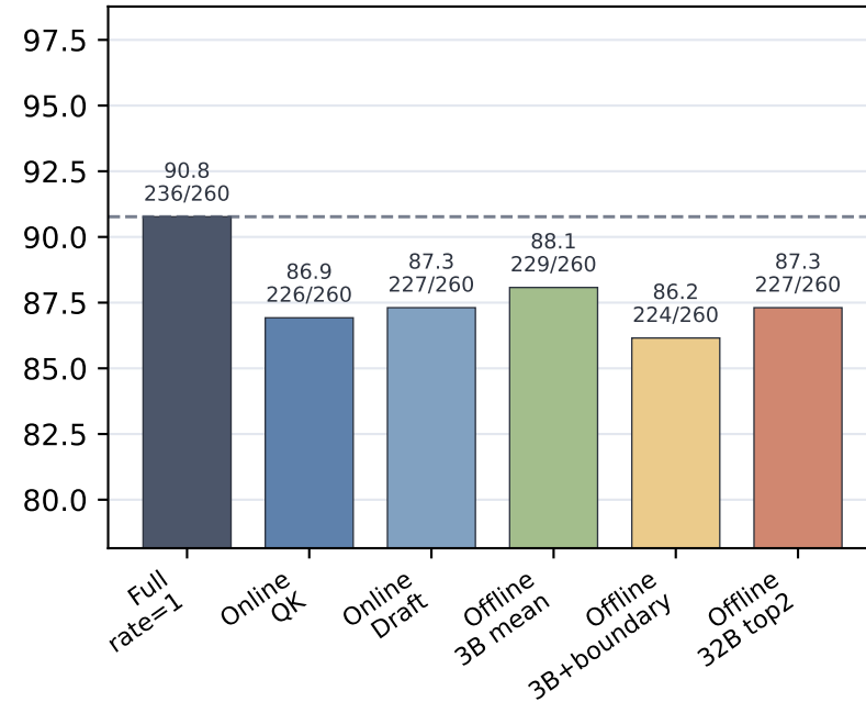
hotpotqa
