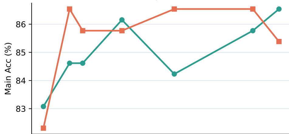
HotpotQA
