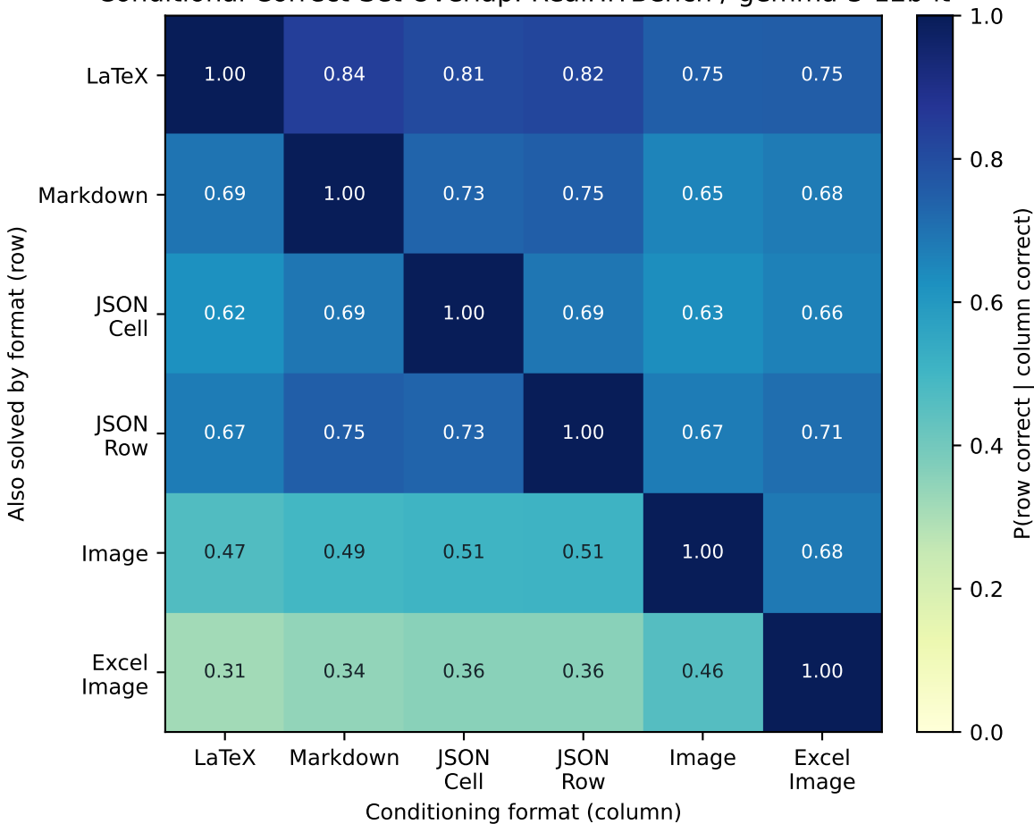
Conditional Correct-Set Overlap: RealHiTBench / gemma-3-12b-it
