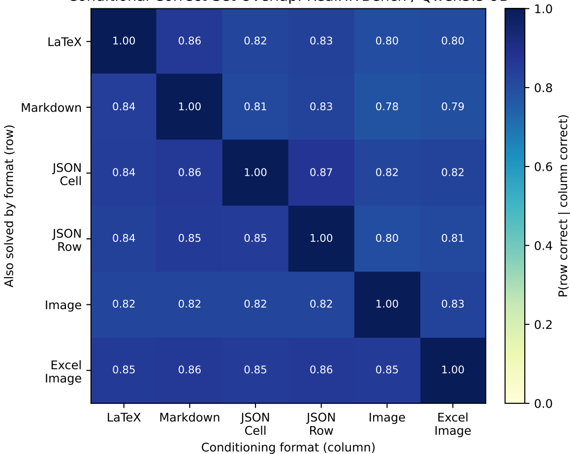
Conditional Correct-Set Overlap: RealHiTBench / Qwen3.5-9B
