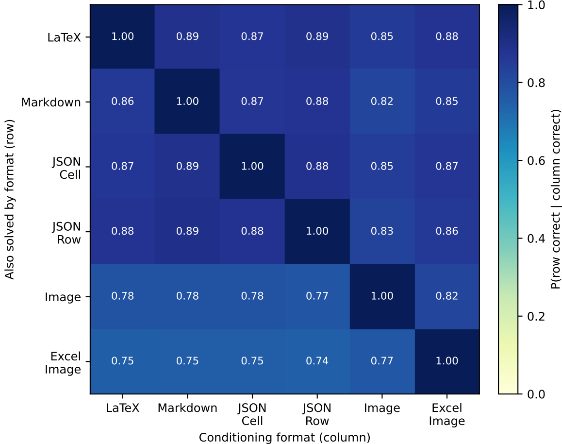
Conditional Correct-Set Overlap: RealHiTBench / Qwen3-VL-30B-A3B-Instruct
