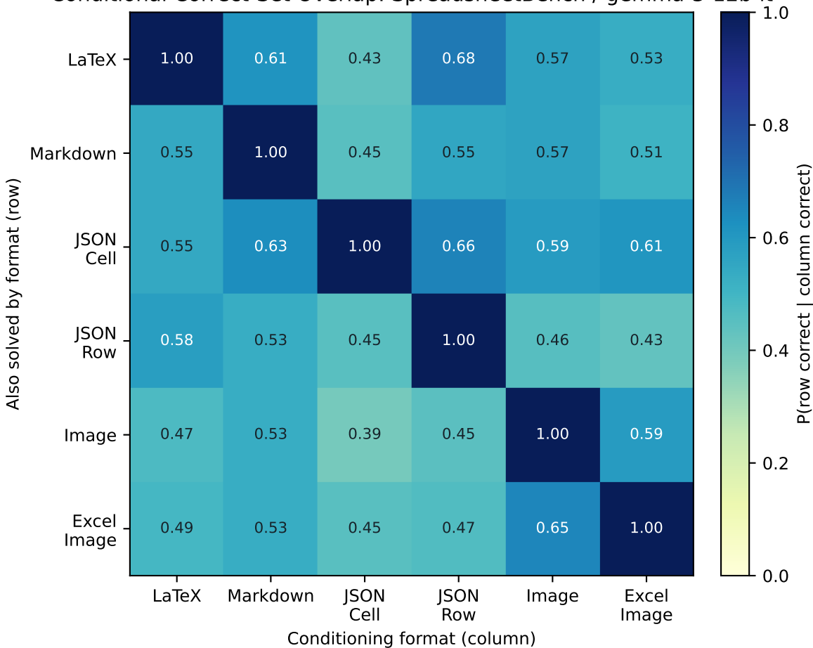
Conditional Correct-Set Overlap: SpreadsheetBench / gemma-3-12b-it
