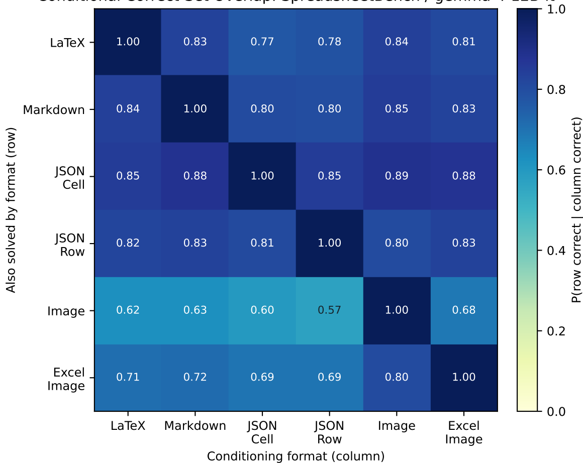
Conditional Correct-Set Overlap: SpreadsheetBench / gemma-4-12B-it
