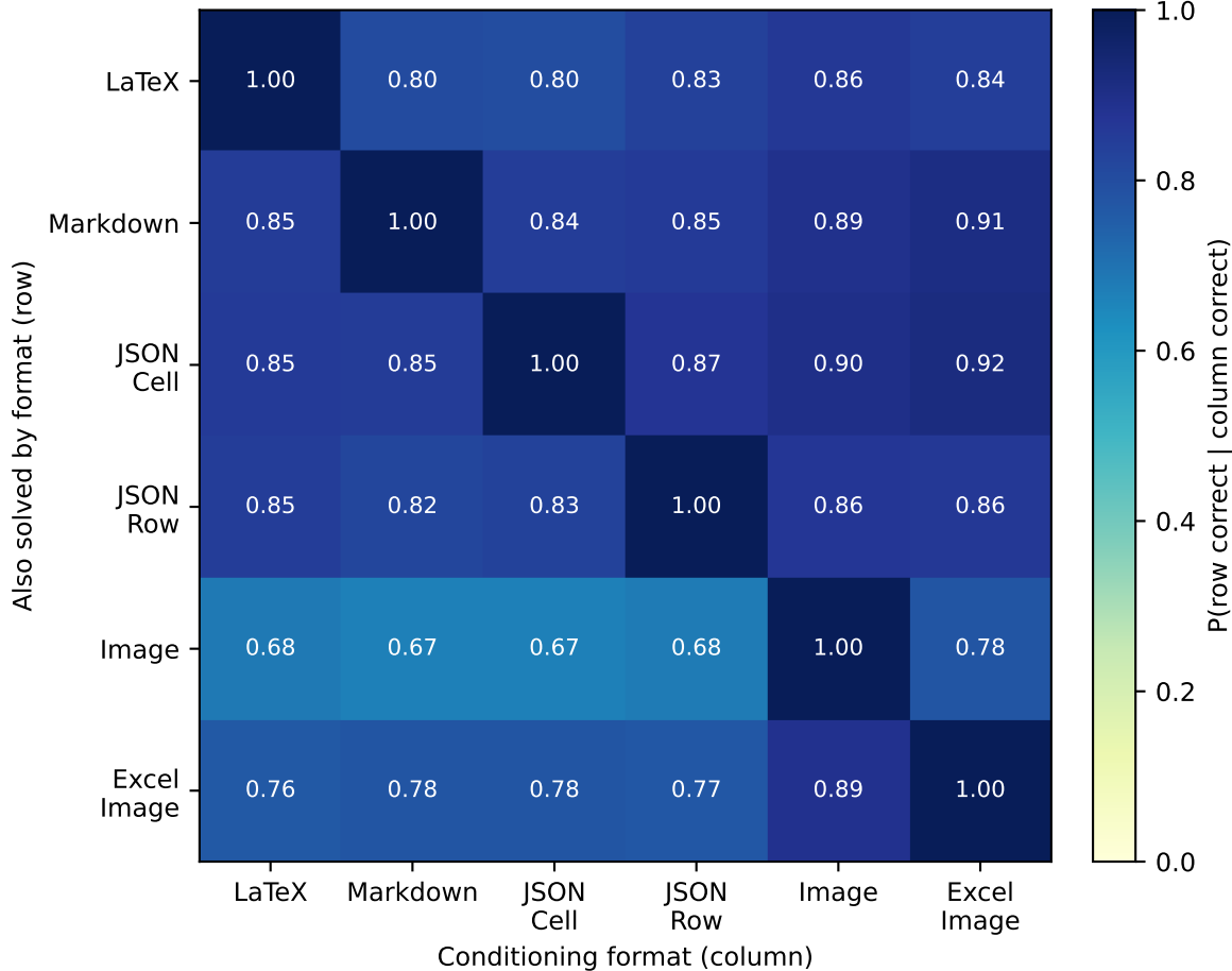
Conditional Correct-Set Overlap: SpreadsheetBench / gemma-4-26B-A4B-it
