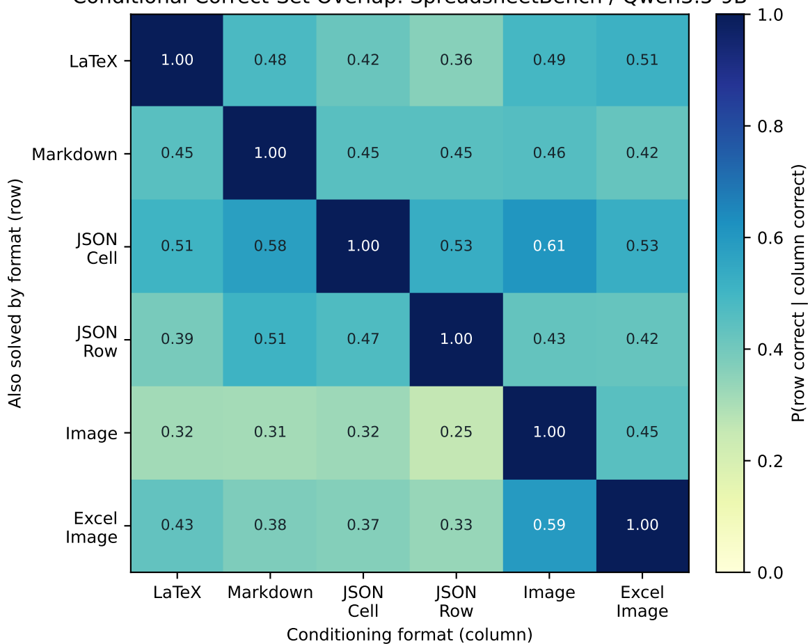
Conditional Correct-Set Overlap: SpreadsheetBench / Qwen3.5-9B
