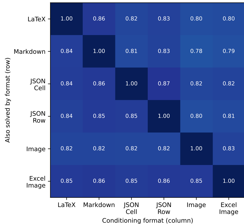
RealHiTBench
