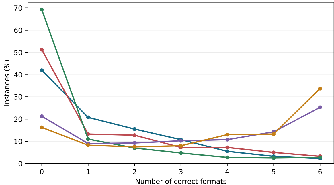
SpreadsheetBench
