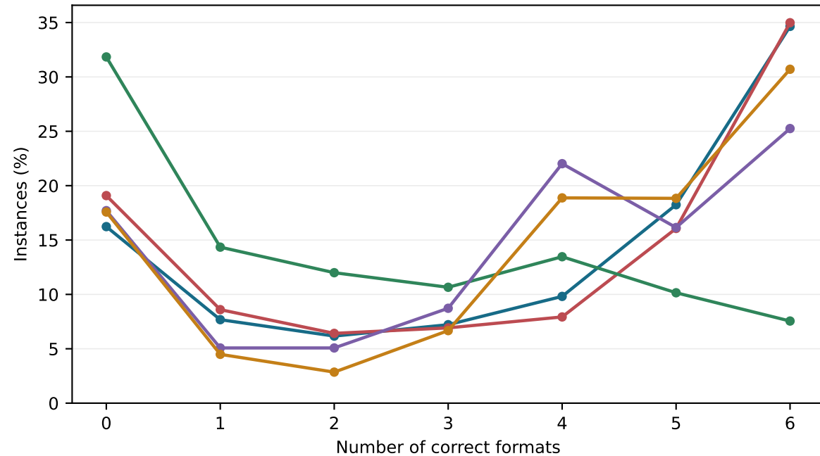
RealHiTBench
