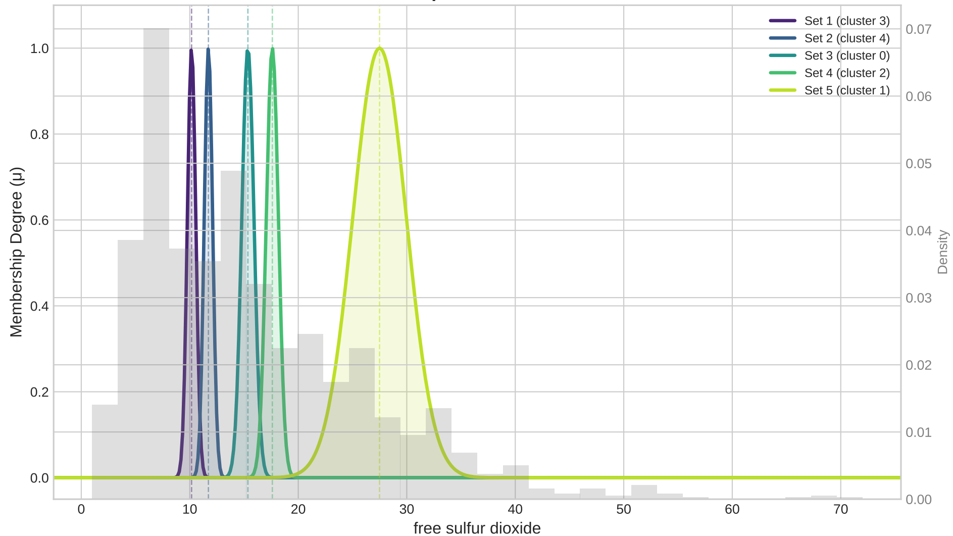
Gaussian Membership Functions: free sulfur dioxide
