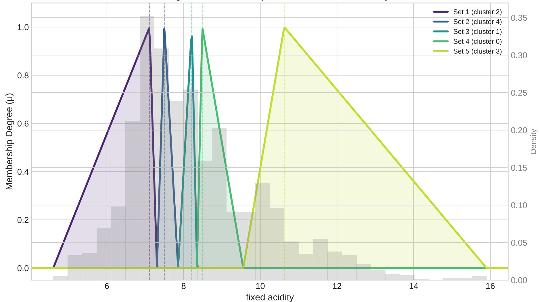
Triangular Membership Functions: fixed acidity
