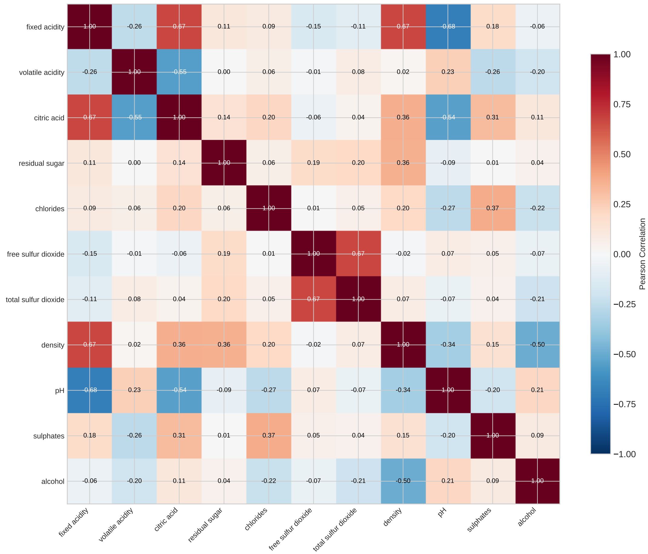
Feature Correlation Matrix
