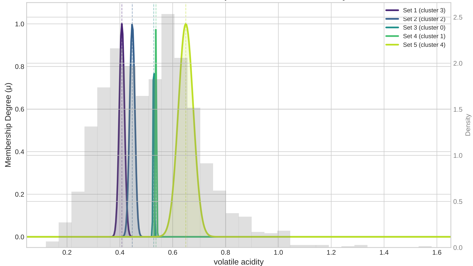
Gaussian Membership Functions: volatile acidity
