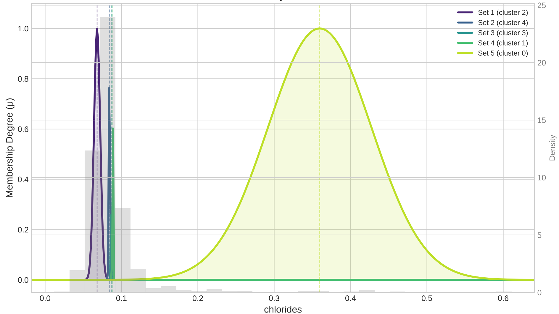
Gaussian Membership Functions: chlorides
