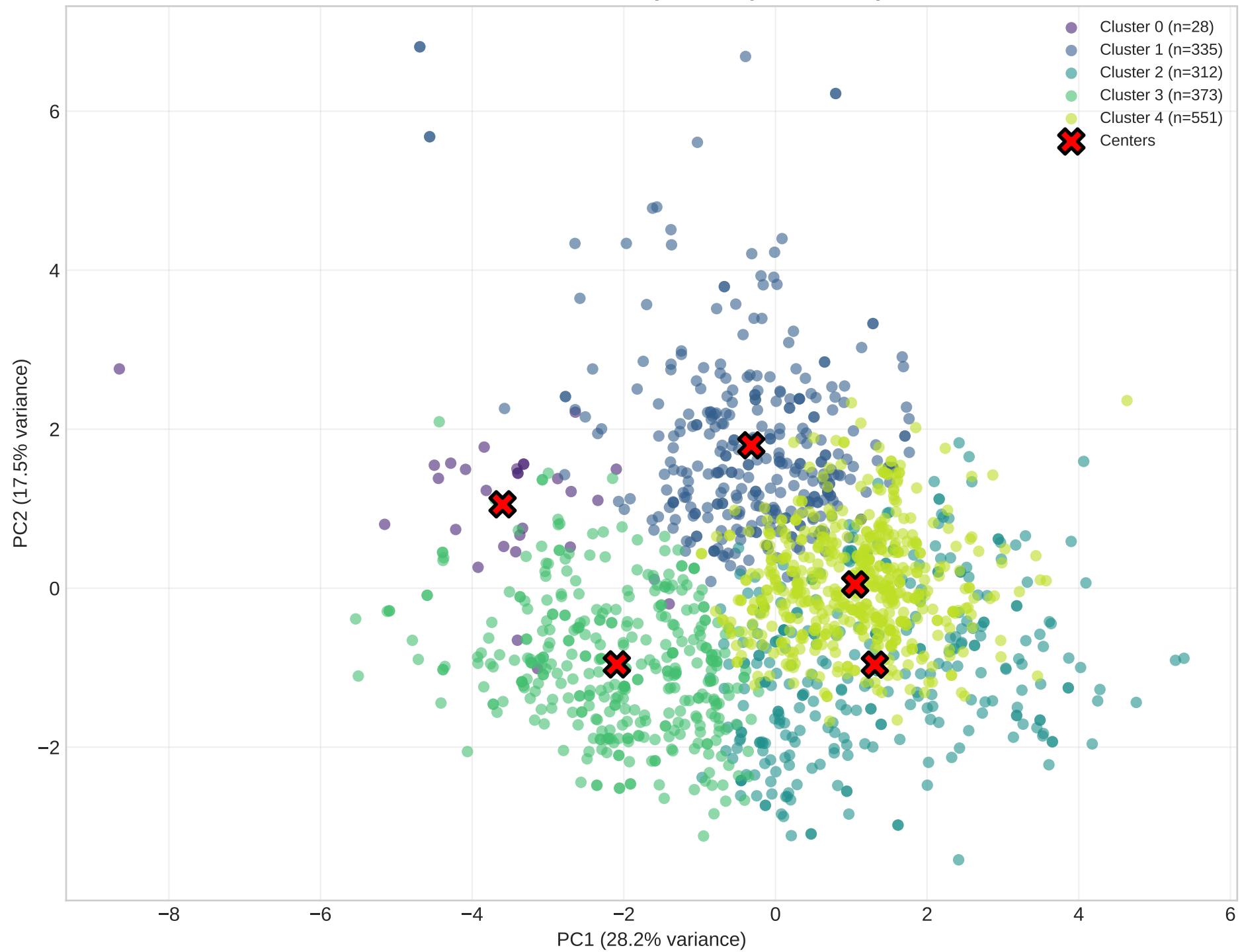
Cluster Visualization (PCA Projection, k=5)
