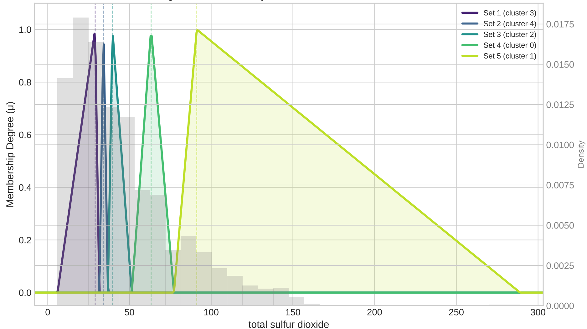
Triangular Membership Functions: total sulfur dioxide
