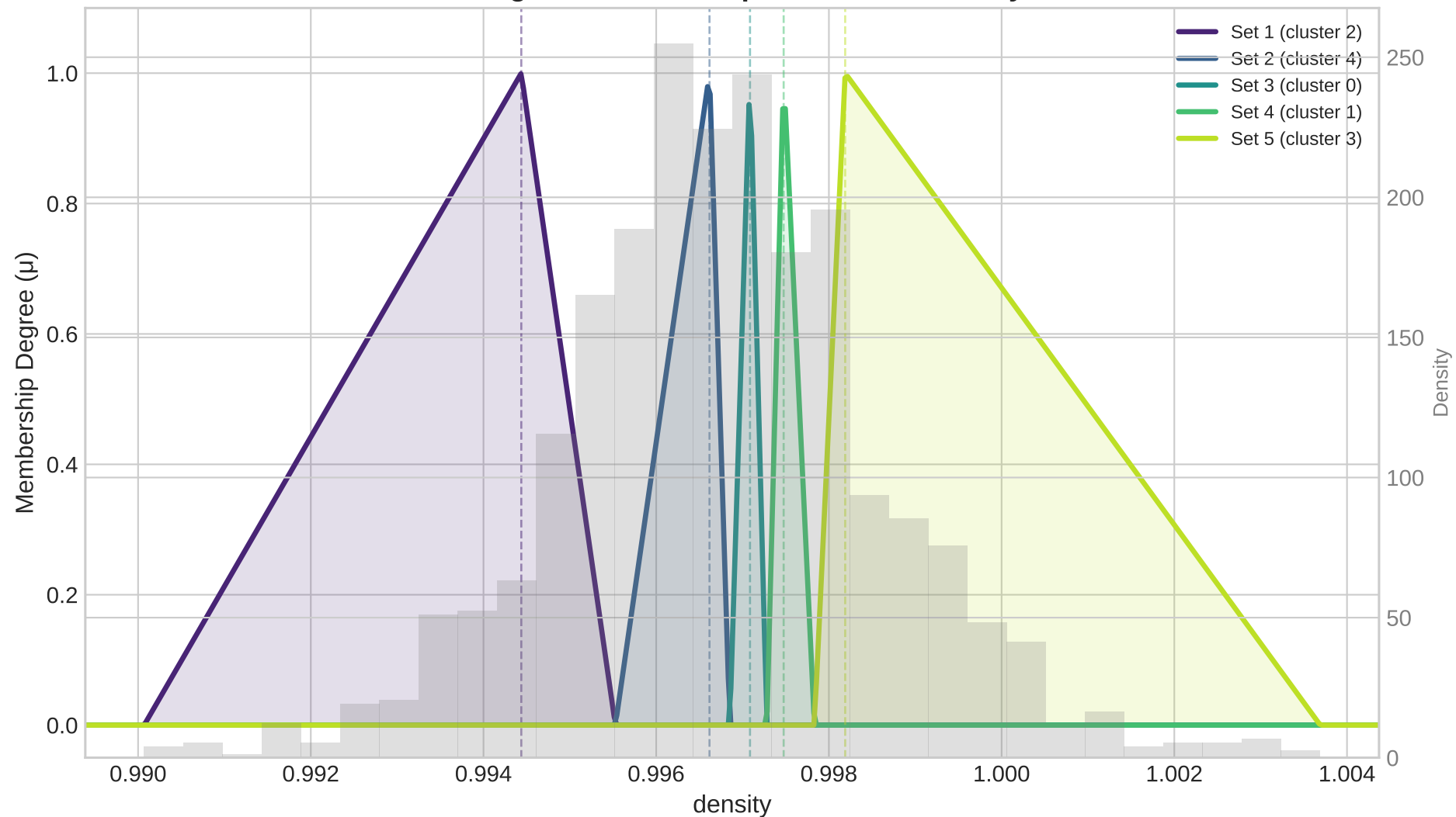
Triangular Membership Functions: density
