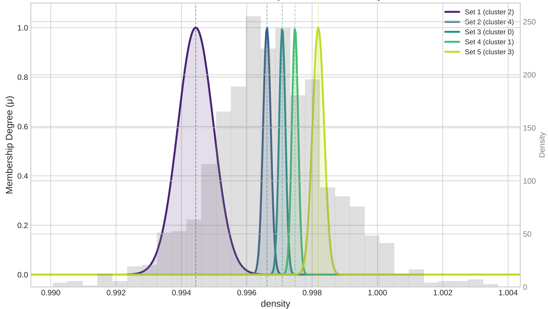
Gaussian Membership Functions: density
