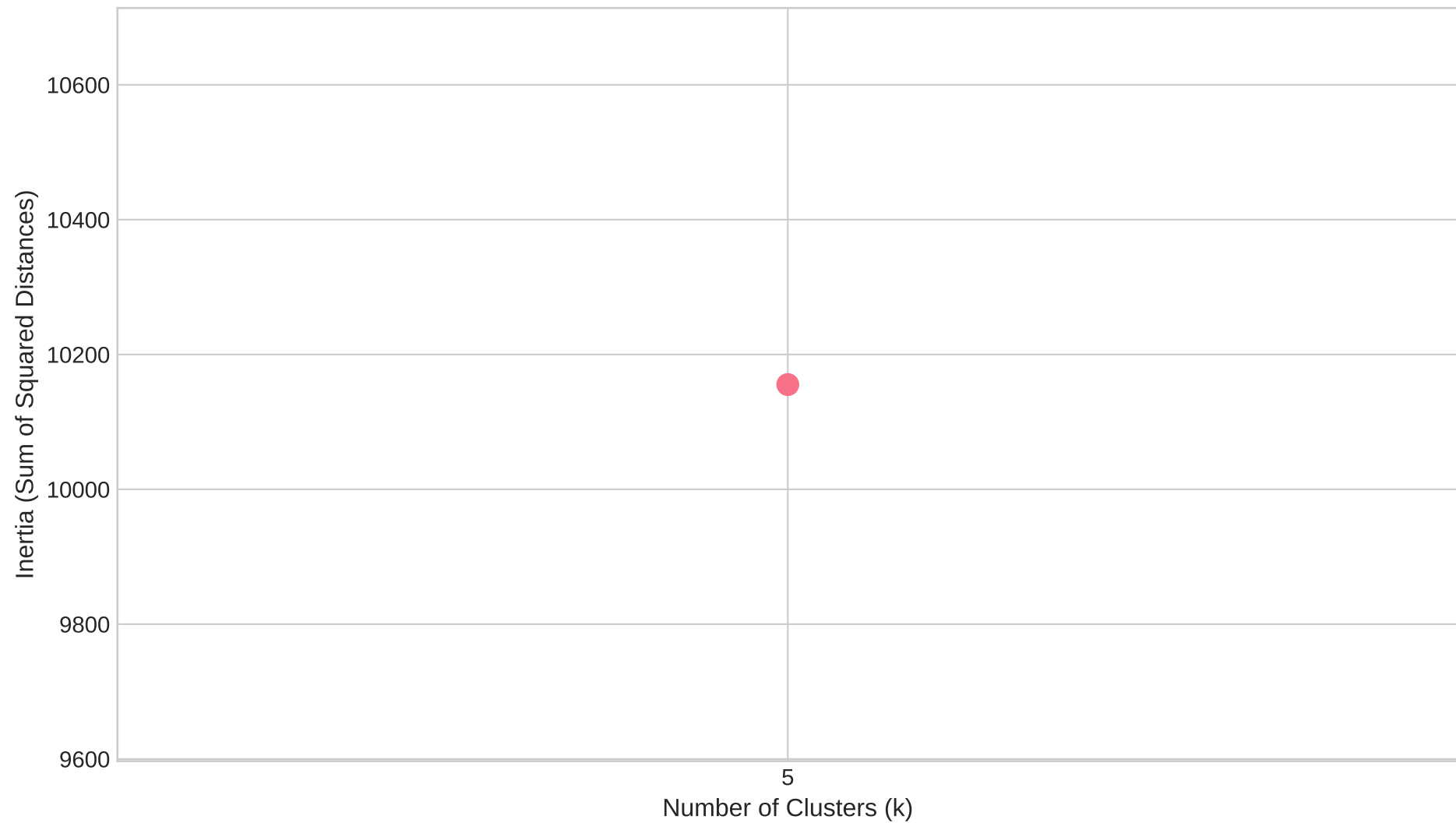
K-means Elbow Curve
