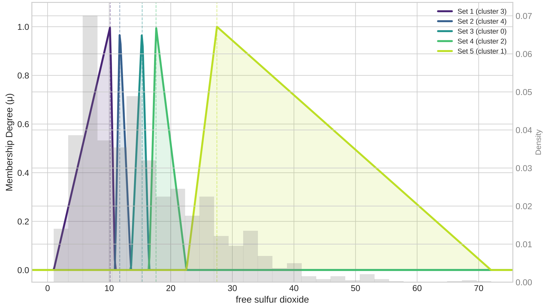
Triangular Membership Functions: free sulfur dioxide
