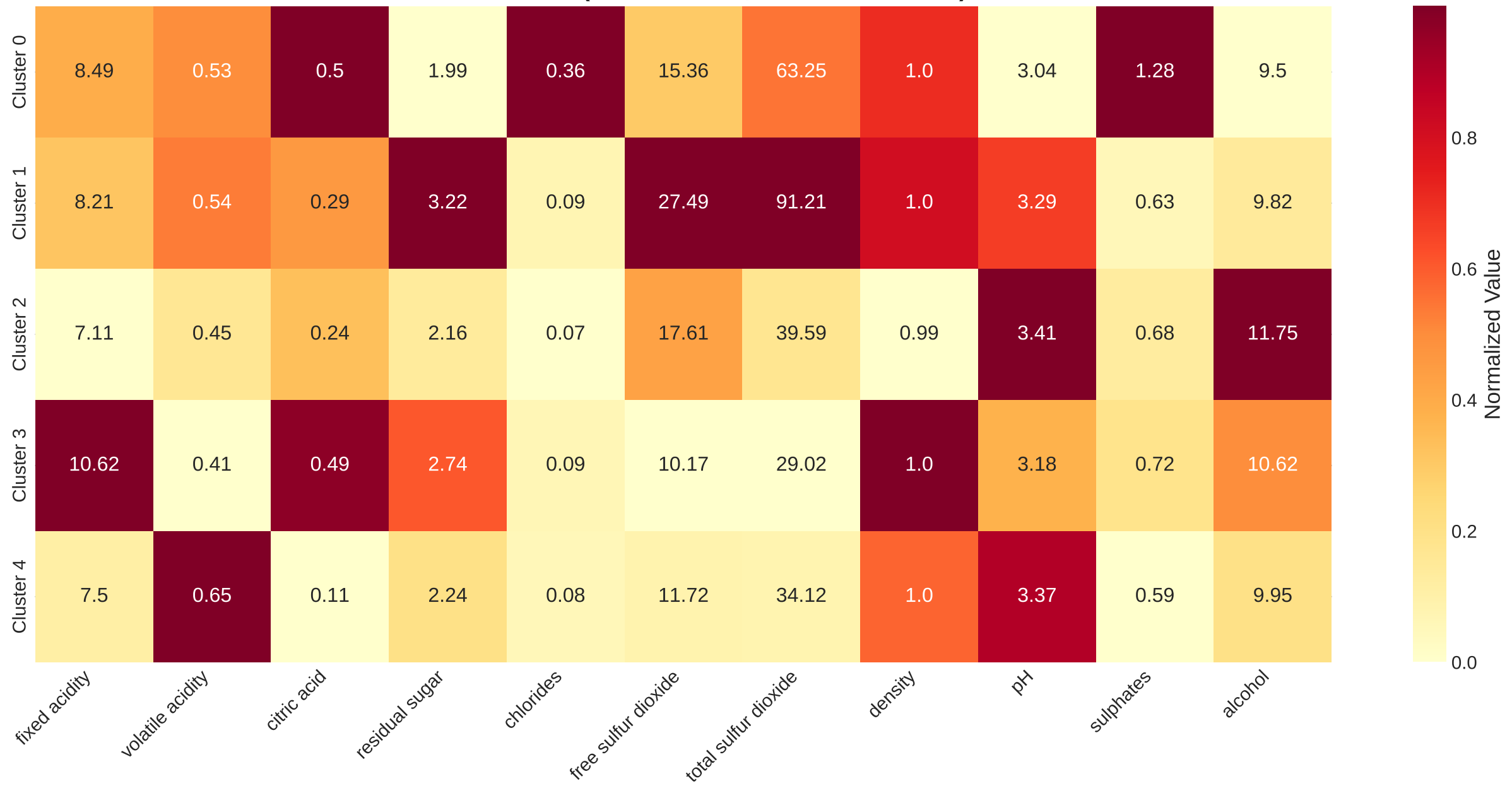
Cluster Centers (values shown, colors normalized)
