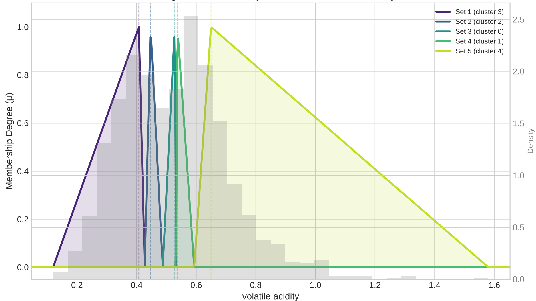
Triangular Membership Functions: volatile acidity
