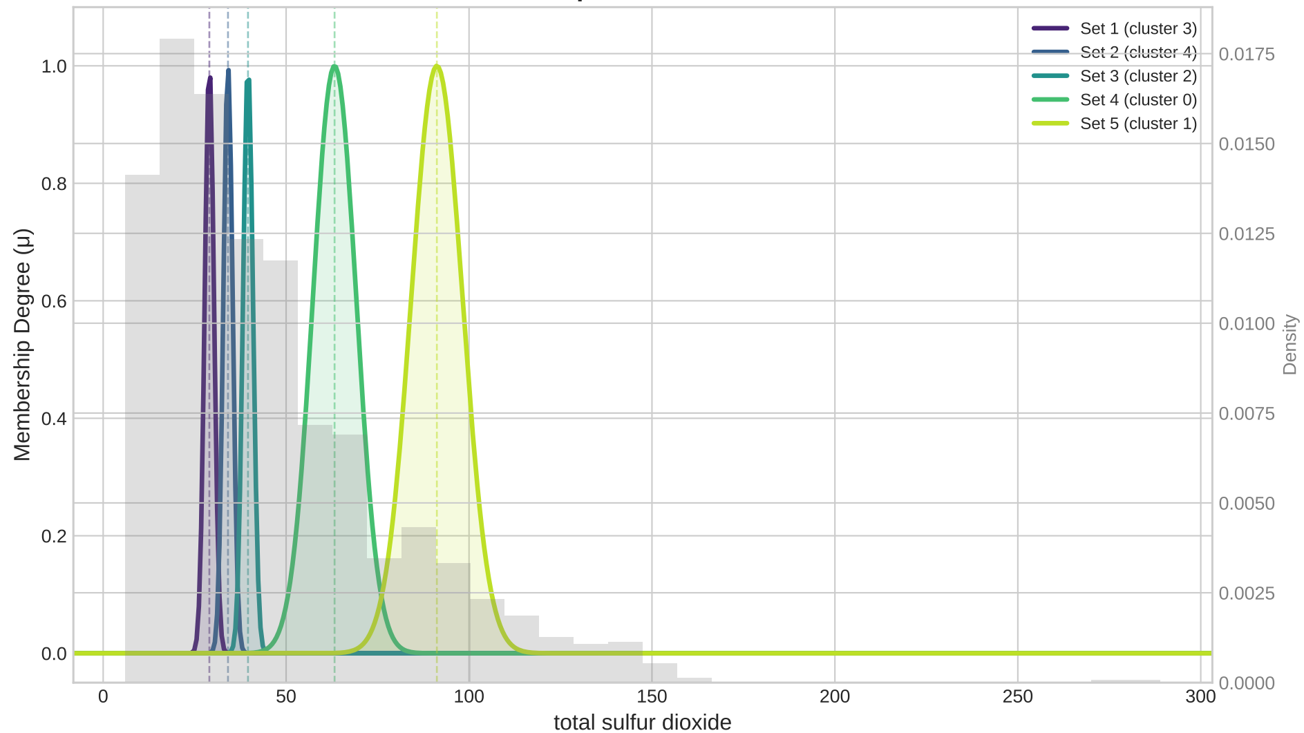
Gaussian Membership Functions: total sulfur dioxide
