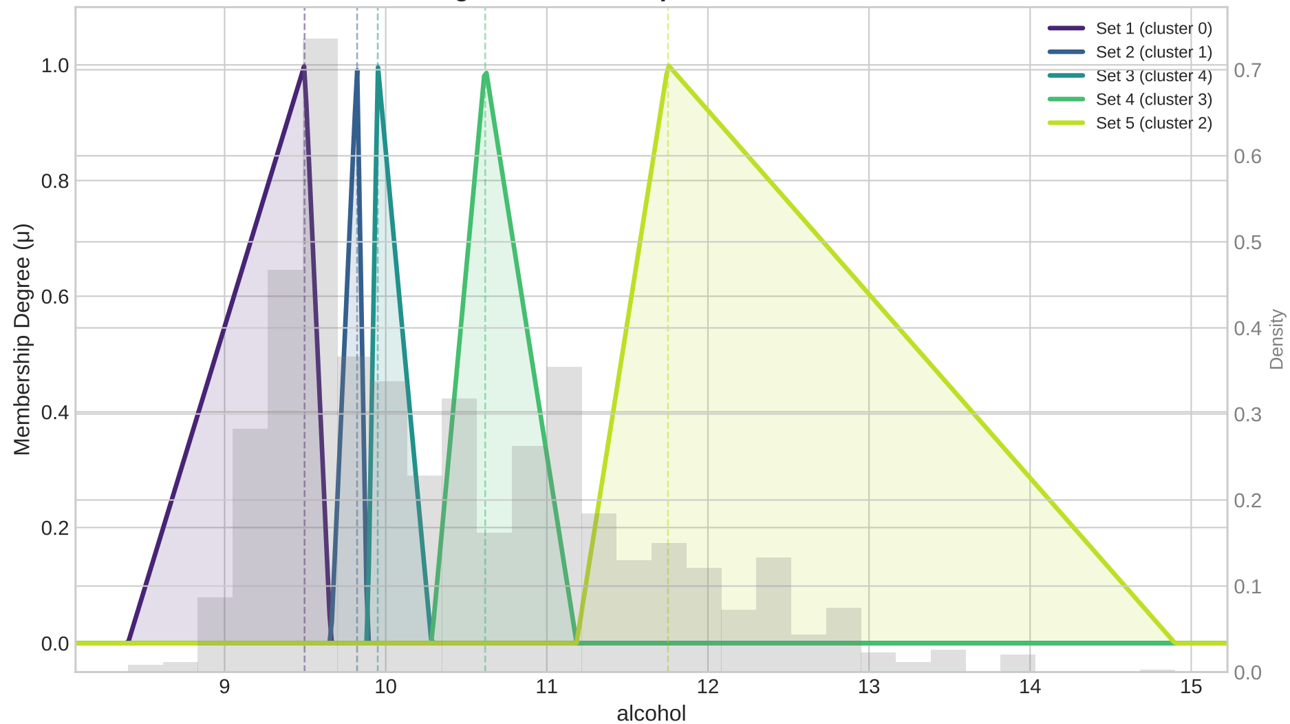
Triangular Membership Functions: alcohol
