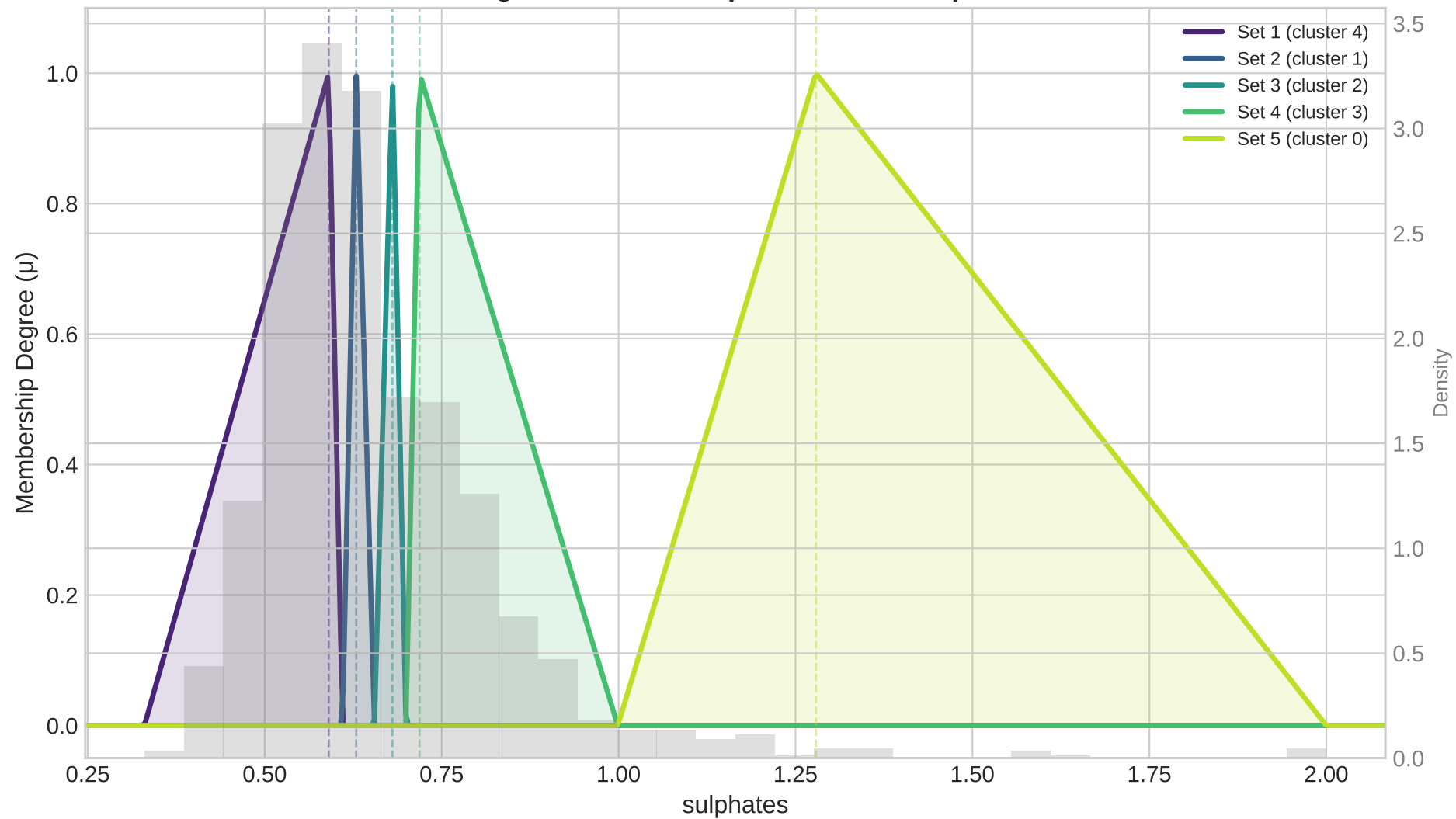
Triangular Membership Functions: sulphates
