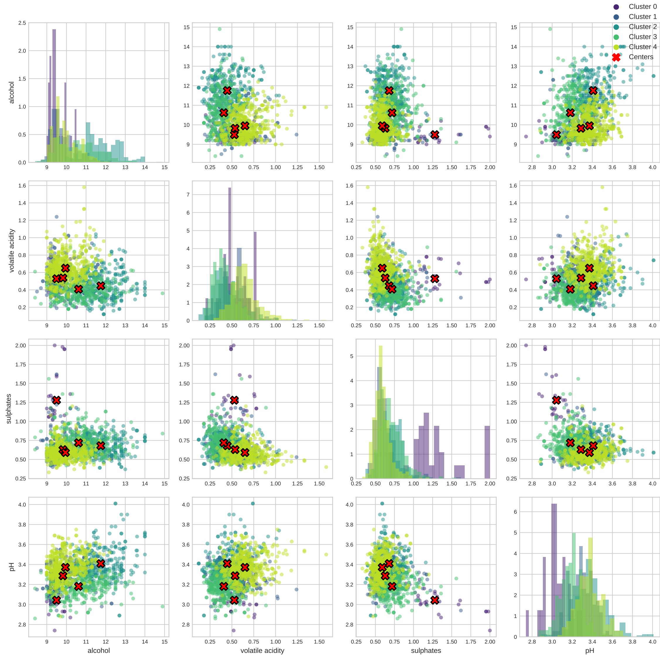
Pairwise Cluster Scatter Plots (k=5)
