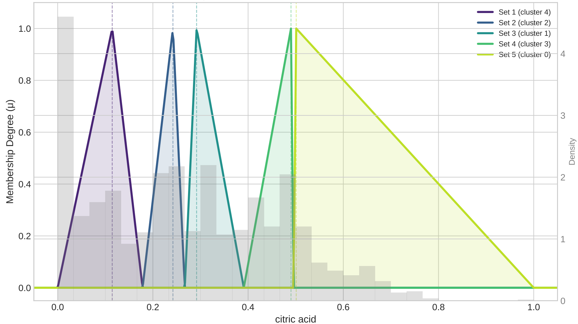
Triangular Membership Functions: citric acid
