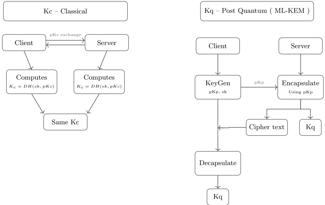
Figure 3.4: Classical and Post-Quantum Key Exchange Mechanisms
