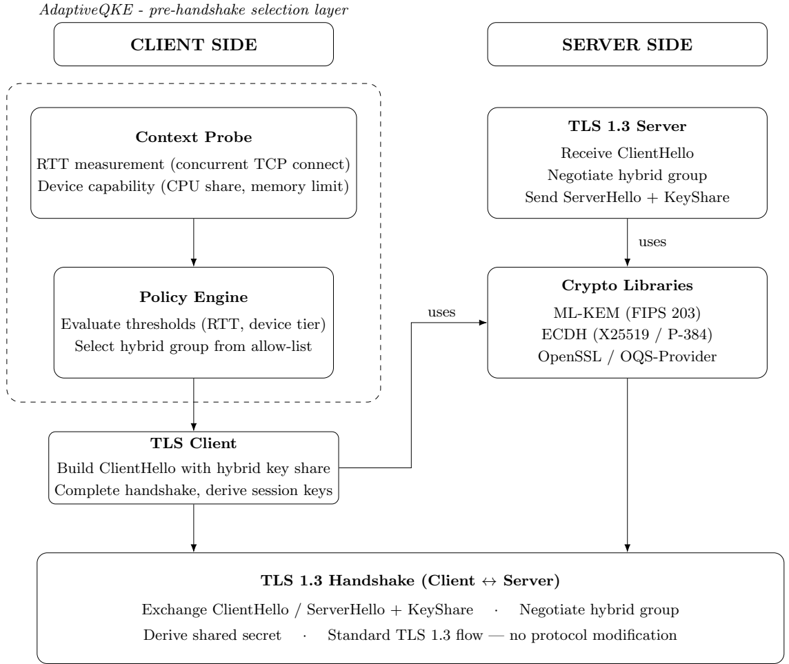
Figure 3.3: System architecture of the proposed AdaptiveQKE framework
