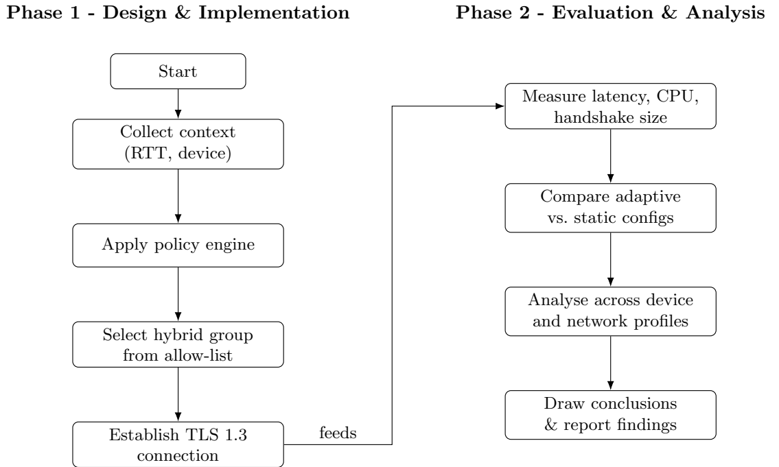
Figure 3.1: High-level overview of the AdaptiveQKE two-phase methodology
