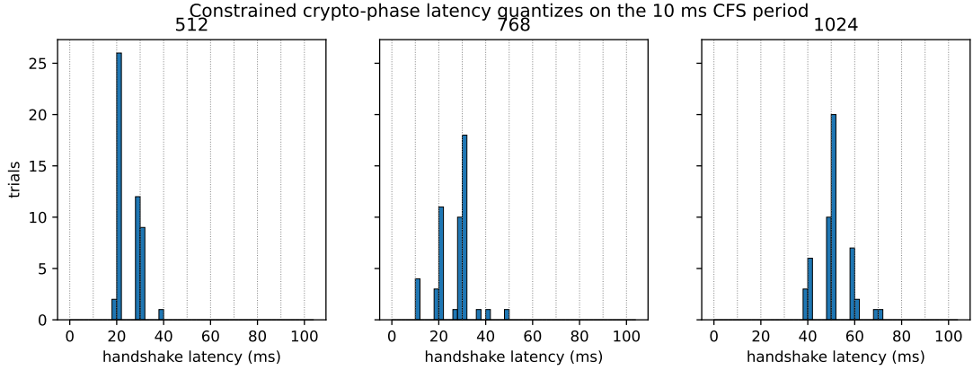
Figure 4.3: Crypto-phase handshake latency on the Constrained device, by hybrid group. Dotted lines mark multiples of the 10 ms CFS scheduling period.
