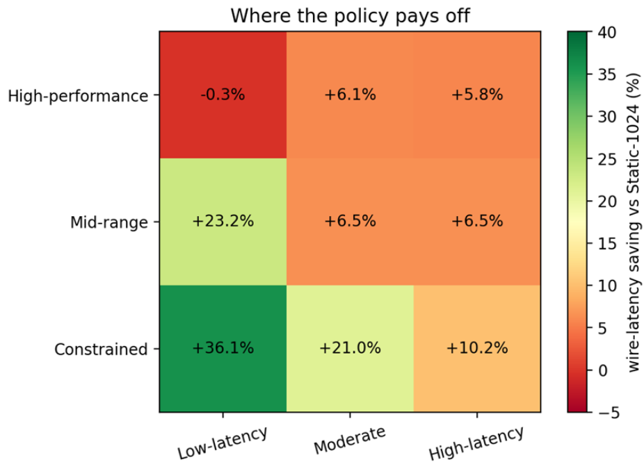
Figure 4.4: Wire-latency savings achieved by Adaptive relative to SecP384r1MLKEM1024 across the nine tested device and network profiles.
