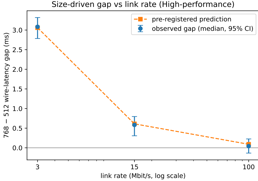
Figure 4.1: Observed Static-768 minus Static-512 wire-latency gap on the high-performance device, by link rate; error bars show 95% confidence intervals.
