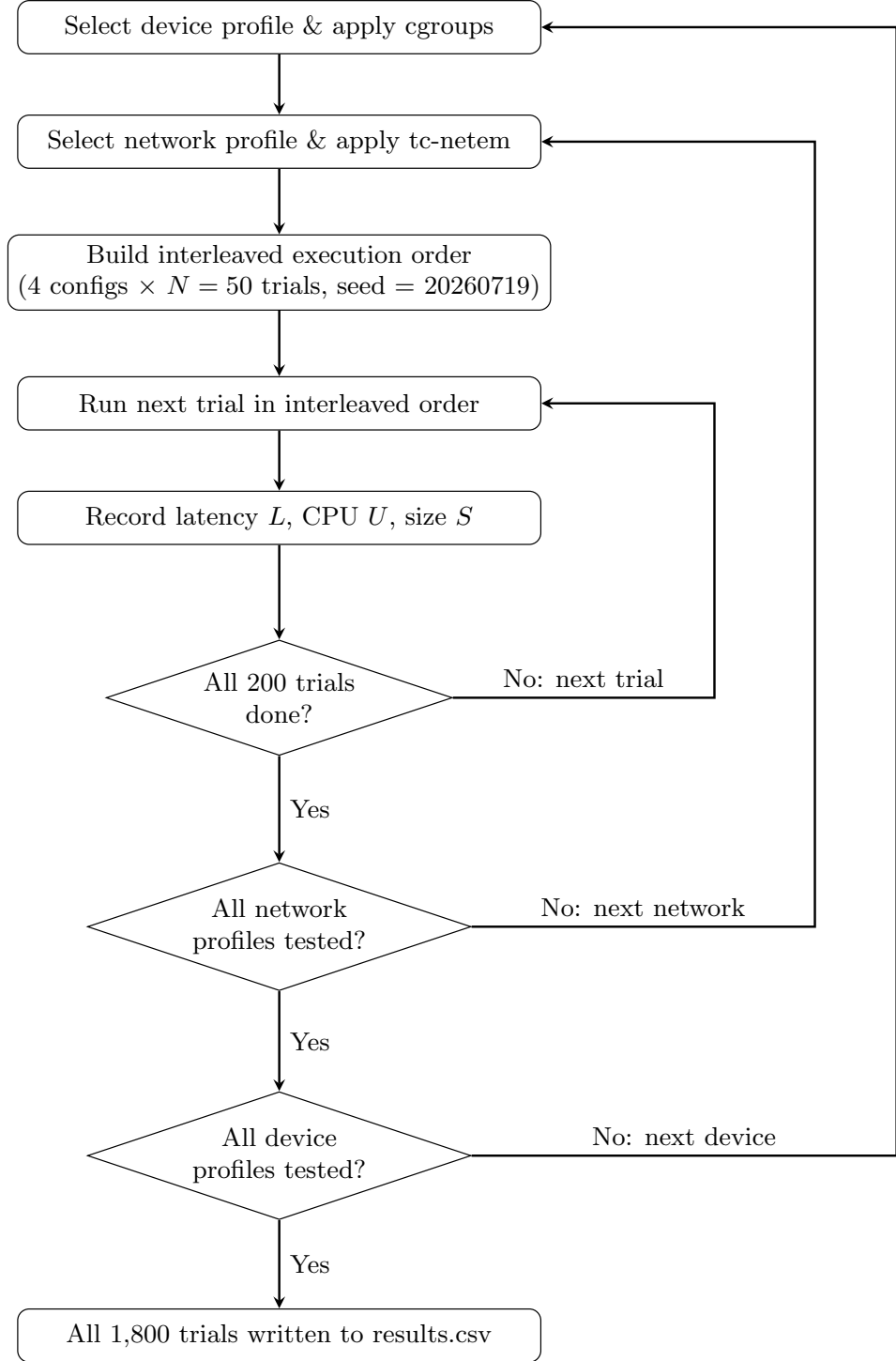
Figure 3.7: Experimental workflow across profile combinations and configurations
