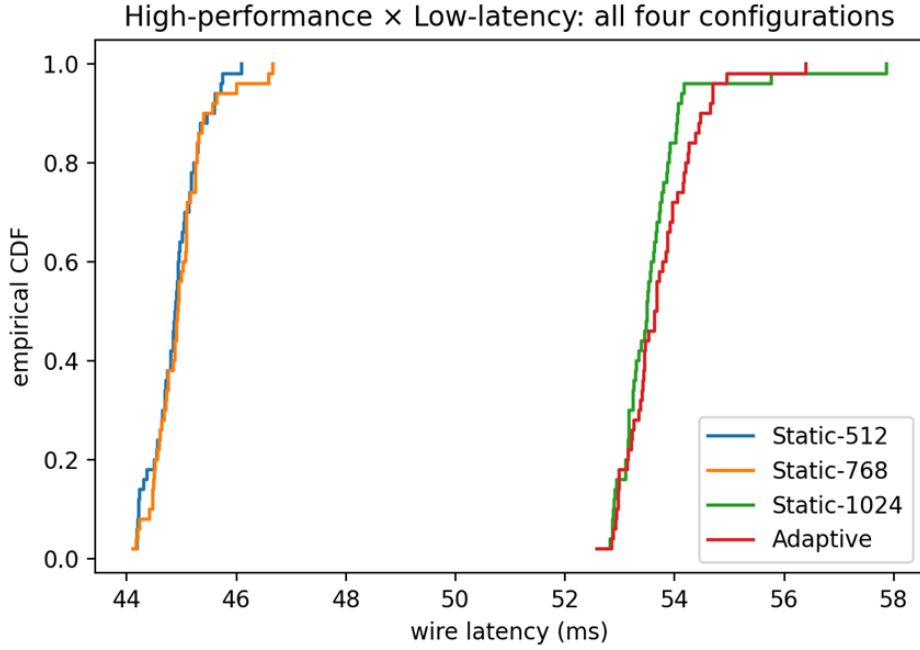
Figure 4.5: Empirical CDF of wire latency under the High-performance and Low-latency profile.
