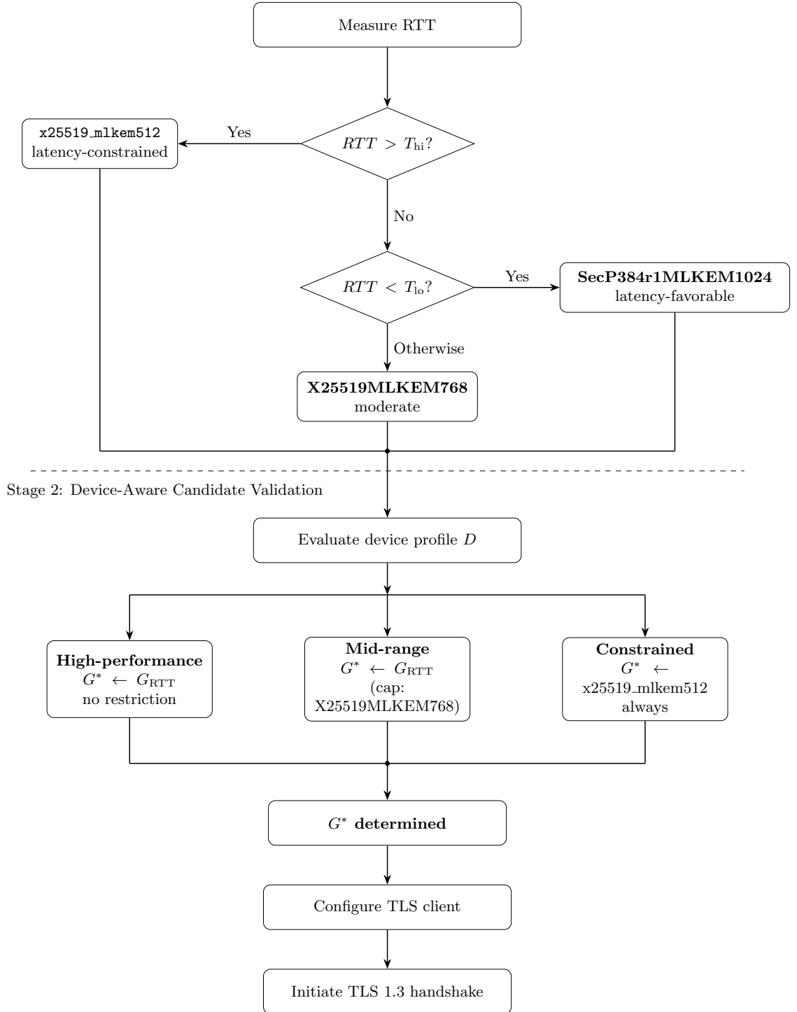
Figure 3.6: AdaptiveQKE policy engine decision flowchart
