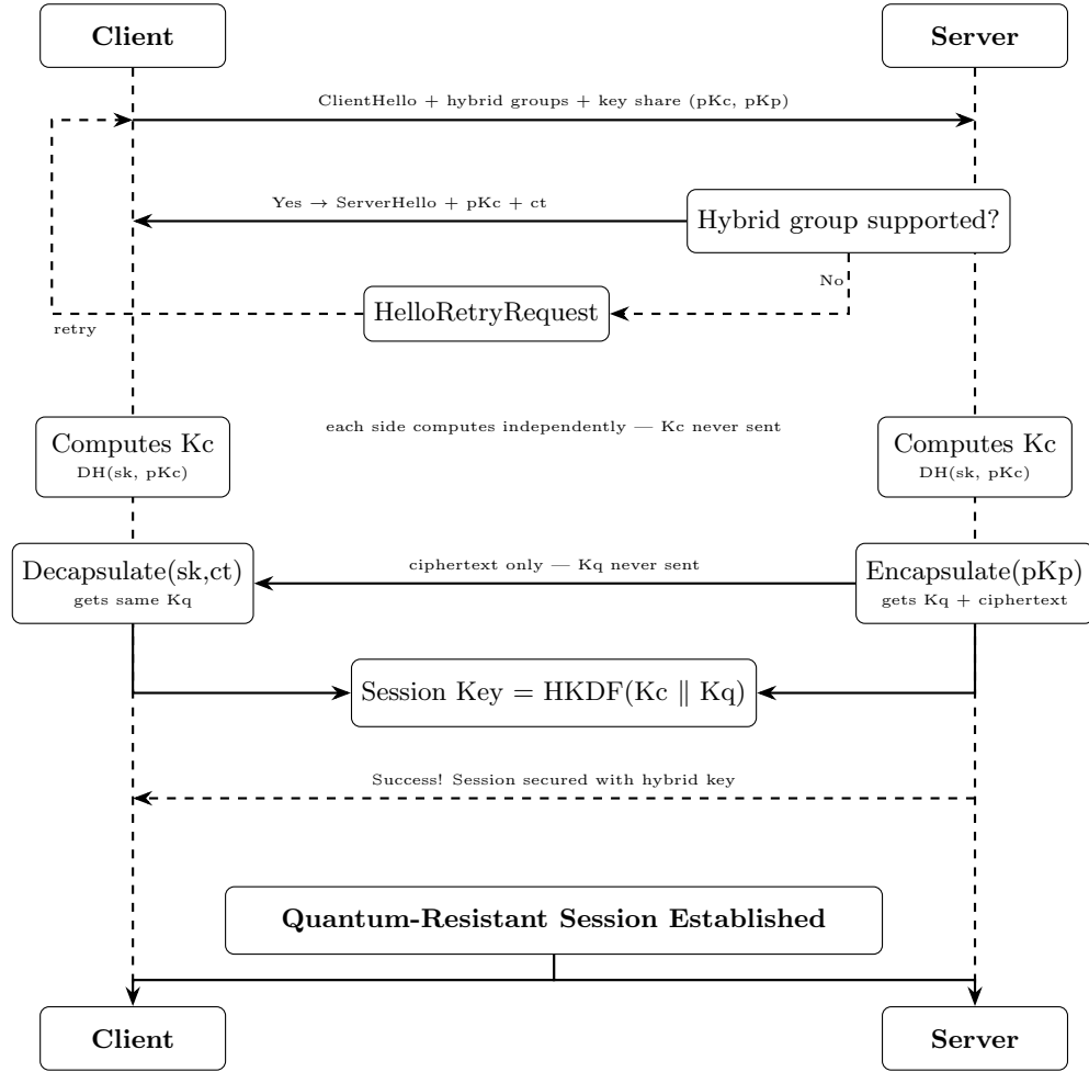
Figure 3.5: Hybrid TLS 1.3 Handshake Protocol Flow [7, 12]
