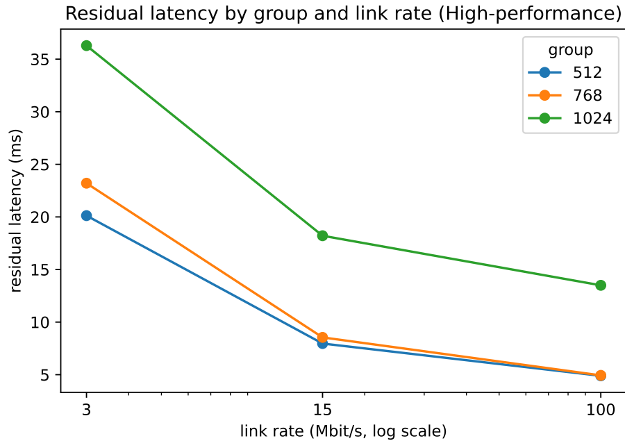
Figure 4.2: Residual wire latency by key-exchange group and link rate on the high-performance device. The link-rate axis uses a logarithmic scale.
