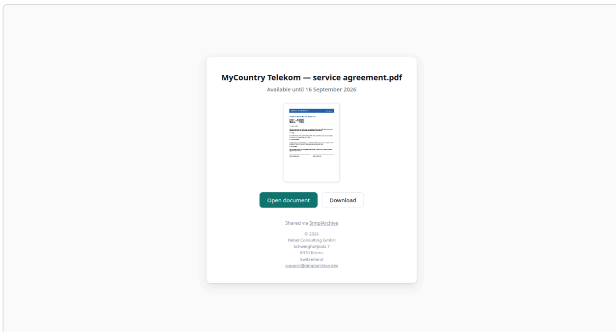
Figure 16: The recipient's view: the document's name and a picture of its first page. This one is a single page, so it carries no page-count marker. No account, one document, nothing else reachable from it.
