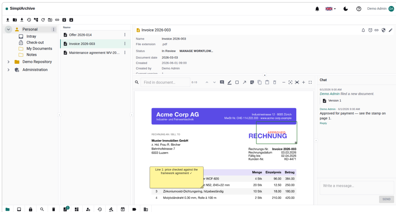
Figure 4: The Personal space expanded: Intray and Check-out sit above your own folders. Drop files on Intray to stage them, or drop an edited working copy on Check-out to bring it back — and drag a document onto Intray to start new work from it as a template.
