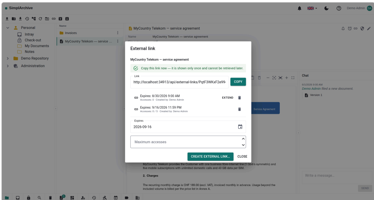
Figure 14: Creating an external link. The URL is revealed once, here, and cannot be retrieved later.
