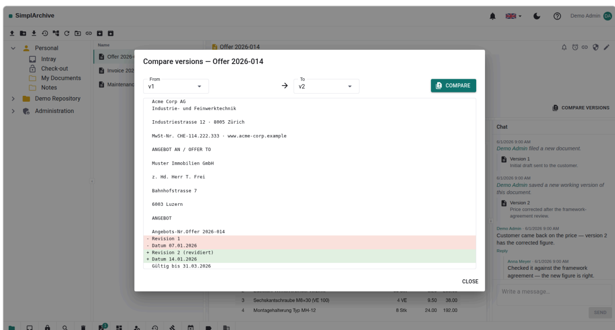
Figure 8: Compare versions: an inline diff of two revisions of a document — added lines marked with +, removed lines with - — so a change between versions is easy to see.
