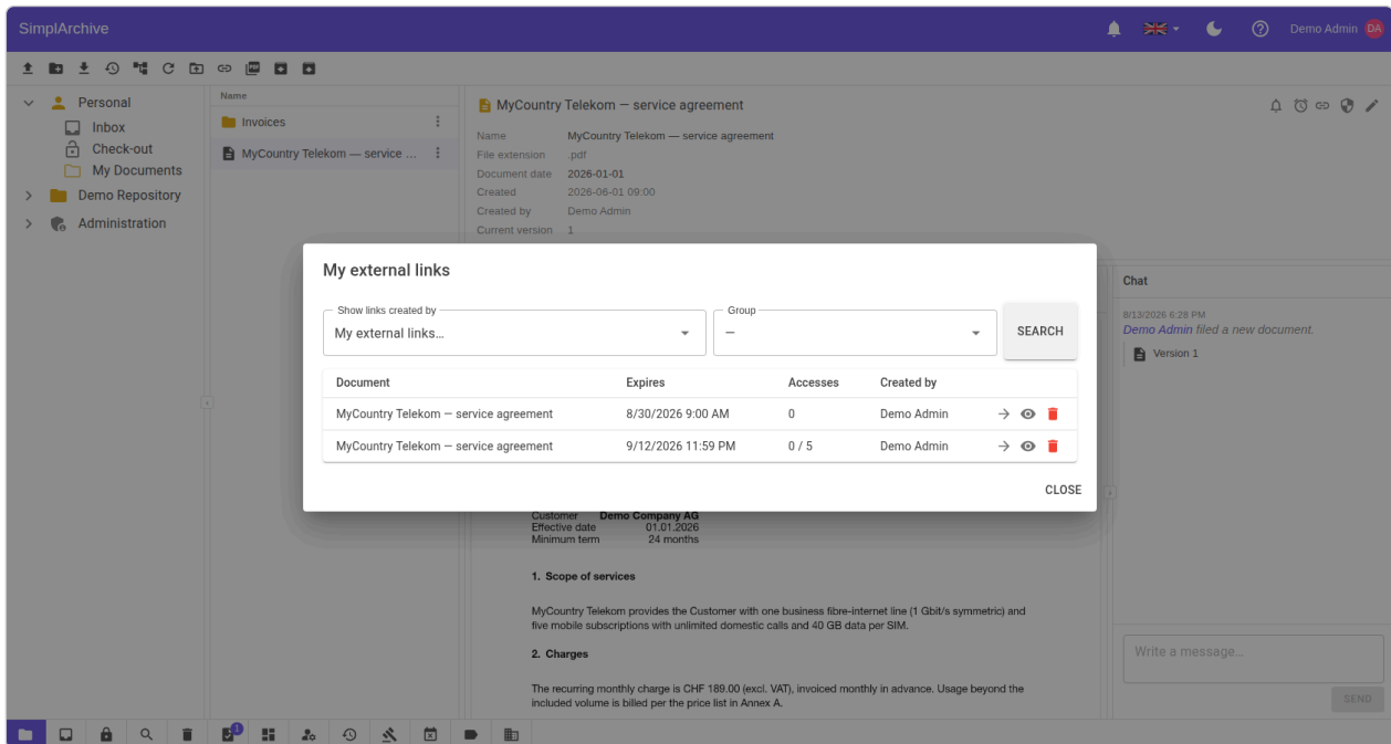
Figure 14: My external links — every live link you have shared, with go-to, details and revoke on each row.
