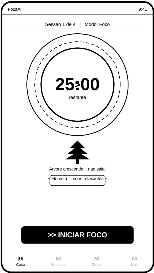
1. Dashboard Principal
