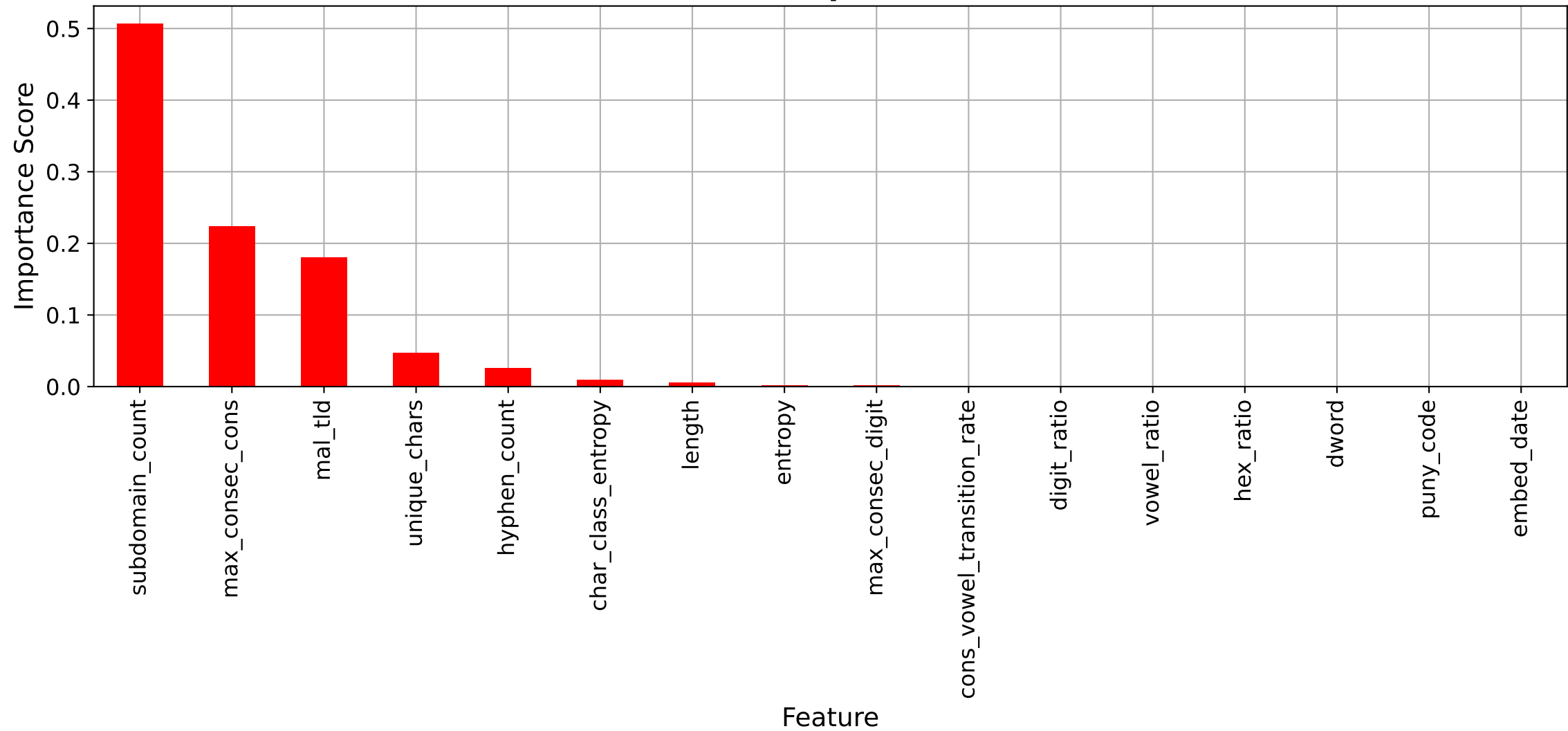
Random Forest Feature Importance (F1 Score Metric)
