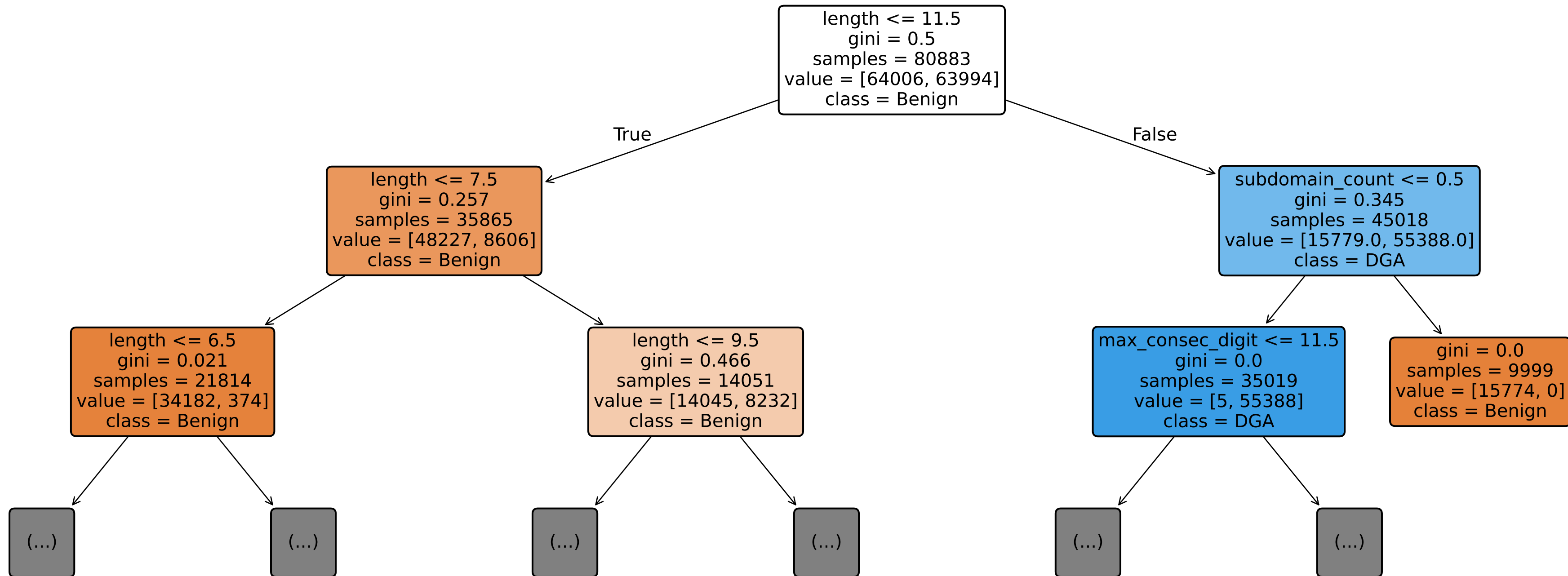
Singular Decision Tree from Random Forest (max_depth=2) (F1 Score Metric)
