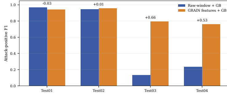
Fig. 3. Representation-controlled comparison. With the same GradientBoosting classifier, same-ID residual features are not better in the closed Test01 setting, but they improve F1 under the three shifted settings. Numbers above each group denote the attack-F1 change of GRAIN-CAN over raw-window statistics.
