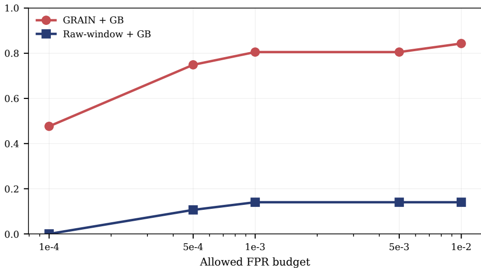
Detection rate at budget
