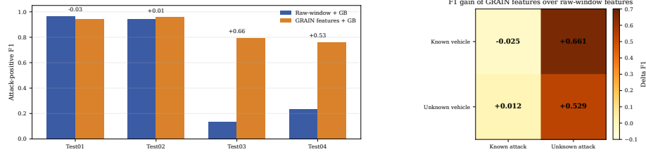
Fig. 3. Representation-controlled comparison. With the same Gradient Boosting classifier, same-ID residual features improve attack-F1 in the three shifted settings, especially when attack families are unknown. The matrix view is categorical rather than temporal and avoids treating Test01–Test04 as a line.
