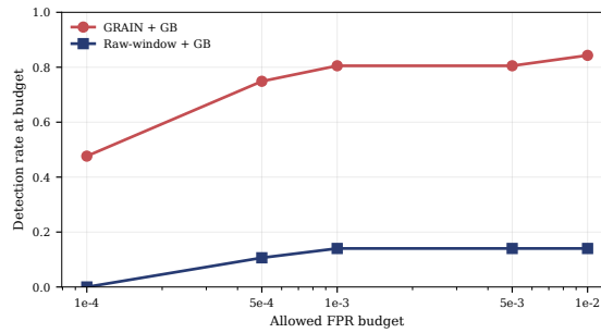
Fig. 5. Supplementary low-FPR operating points on Test04. Same-ID residuals preserve higher attack recall than raw-window statistics under matched false-alarm budgets.
