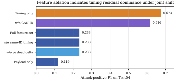
Fig. 4. Feature ablation on Test04. Timing residuals dominate under joint shift; raw-ID and payload-heavy variants are less robust.
