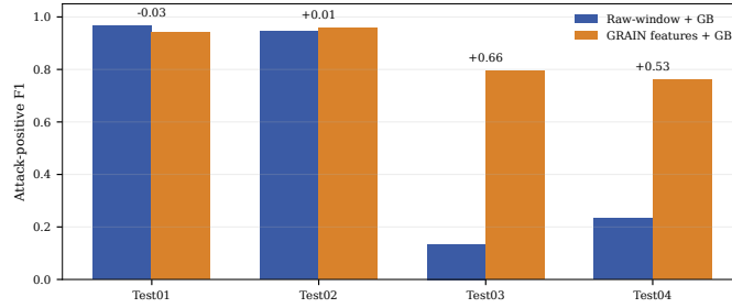
Fig. 3. Representation-controlled comparison. With the same Gradient Boosting classifier, same-ID residual features are not better in the closed Test01 setting, but they improve attack-F1 under the three shifted settings. Numbers above each group denote the attack-F1 change of GRAIN-CAN over raw-window statistics.
