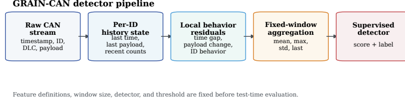
Fig. 2. GRAIN-CAN detector pipeline. The representation is built before the window is formed: raw frames update a per-ID history state, local residuals are extracted from same-ID history, and the resulting frame features are aggregated for supervised classification.
