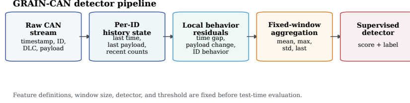
Fig. 2. GRAIN-CAN detector pipeline. The representation is built before the window is formed: raw frames update a per-ID history state, local residuals are extracted from same-ID history, and the resulting frame features are aggregated for supervised classification.
