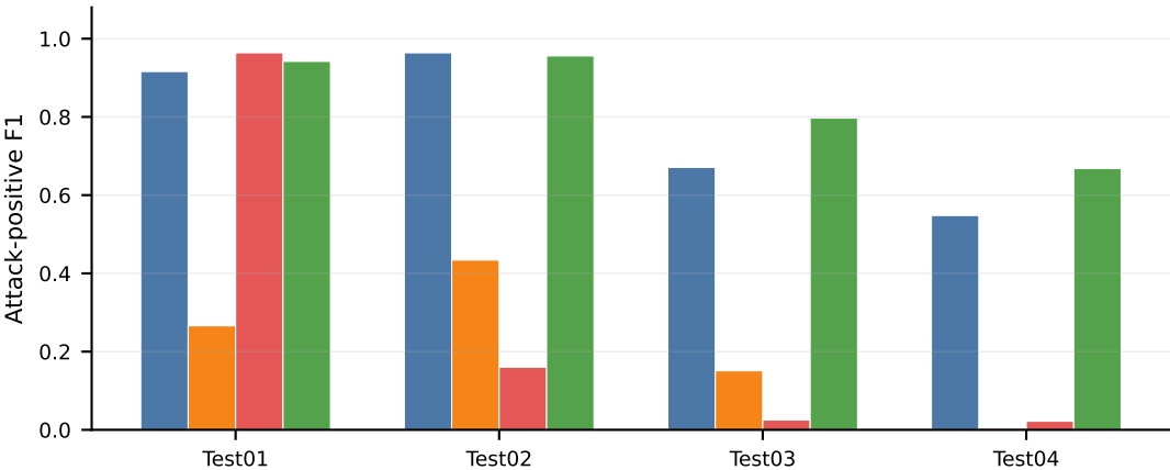
GB-sample MLP Raw-Trans GRAIN-W100 Cross-shift detection under conventional attack-positive F1
