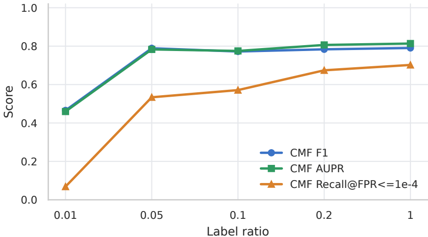
ROAD few-label behavior
