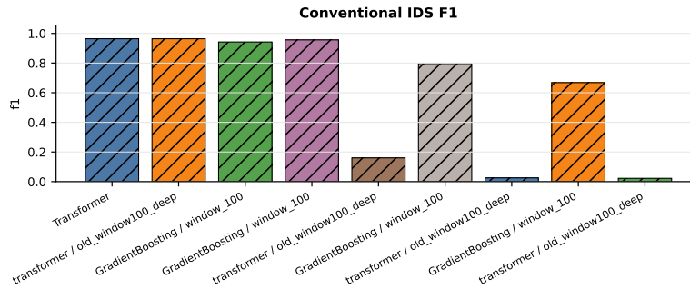
Fig. 3. Representative conventional F1 results. The chart uses reproduced or locally computed rows only.
