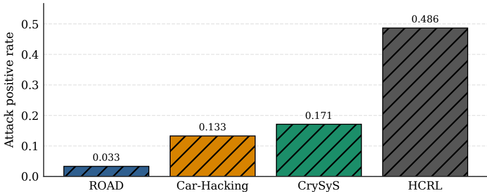
External sanity availability and label-balance audit
