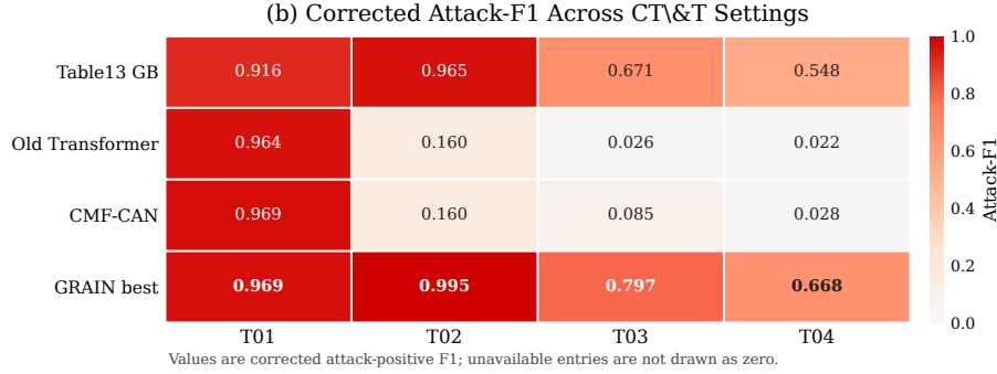
Figure 3: Corrected benchmark across CT&T settings. The attack-centric view distinguishes genuine attack detection from normal-dominated aggregate scores.
