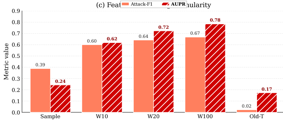
Figure 5: Feature-preserving granularity evidence. Aggregate windows help when they preserve causal timing and payload signals rather than hiding rare evidence.
