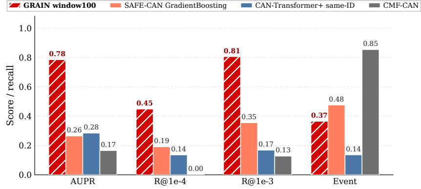
Figure 6: Completed low-FPR evidence after recomputing from available score dumps. High event recall alone can be misleading when score separation and low-FPR recall are weak.
