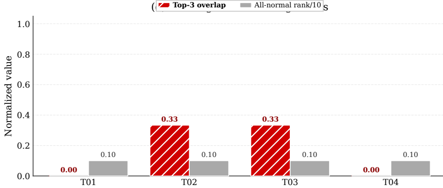
Figure 4: Ranking inversion under aggregate and attack-centric metrics. Normal-dominated metrics can change which IDS appears best.
