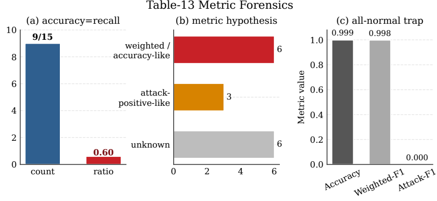
Figure 2: Metric forensics case study. High aggregate scores under rare attacks can be consistent with normal-dominated metrics; they should not be interpreted as attack-positive F1 without confusion matrices.
