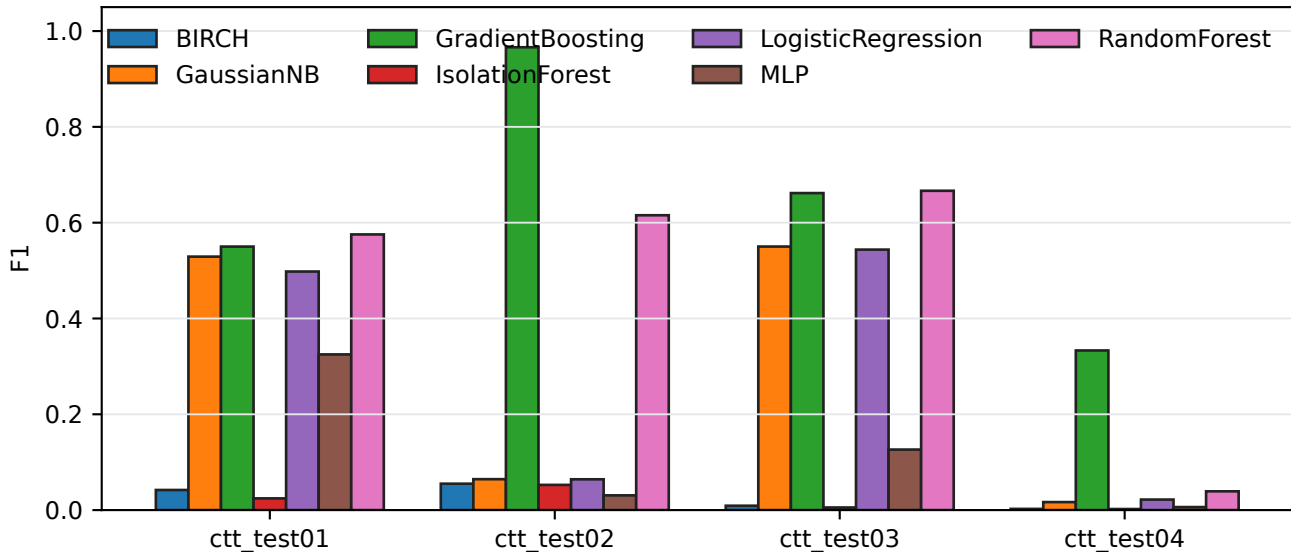
Official sample-level ML
