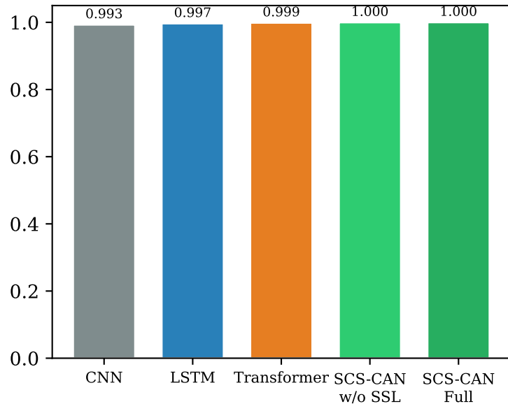
HCRL-CH
