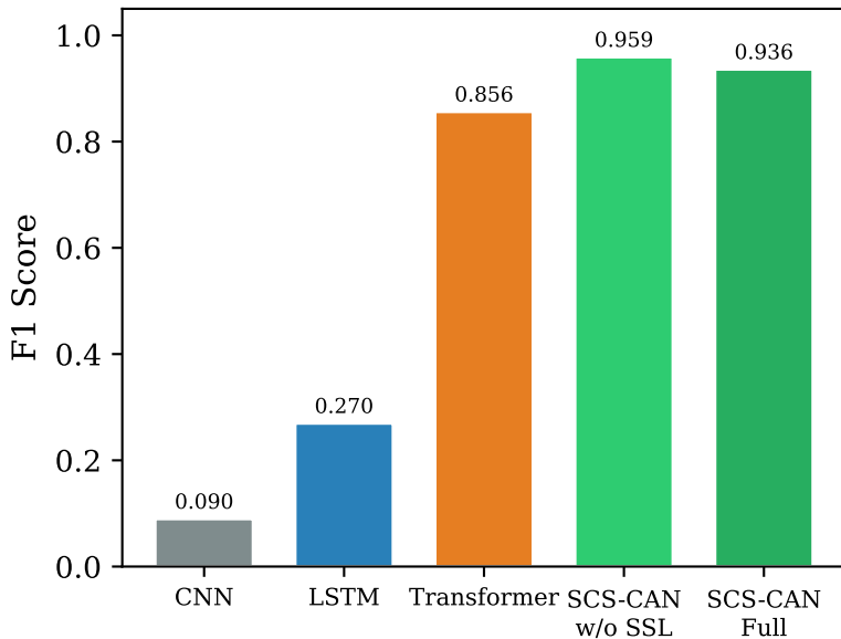
ROAD
