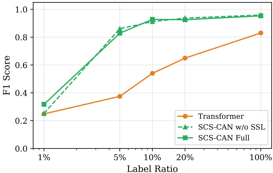
Few-Label Performance (ROAD)
