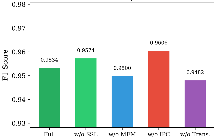
Ablation Study (ROAD)
