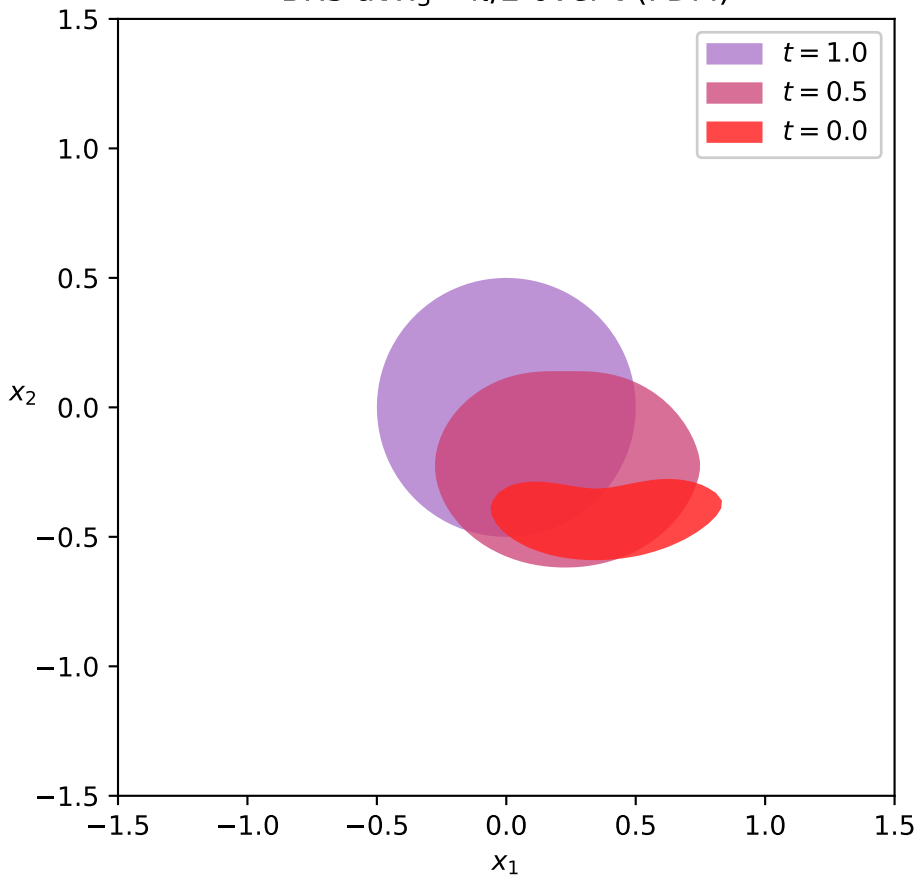
BRS at x_3 = \pi/2 over t (FDM)
